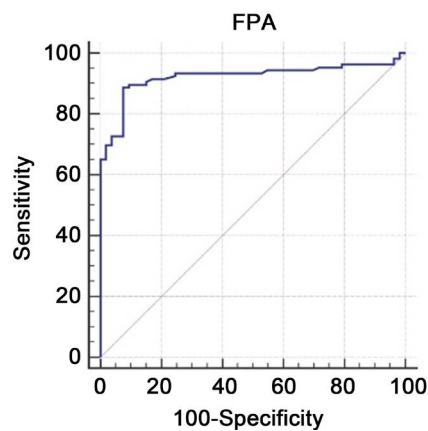
Figure 1. Curve and area under the curve for the fluorescence polarization assay.
