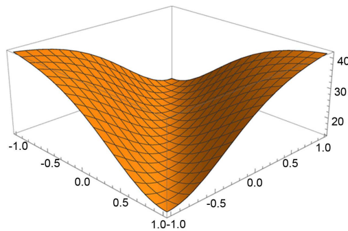
Figure 1. Simulation u_1(x, t) of Equation (7) with \alpha = -1 , \beta = 2 , \gamma = 0.4 , \kappa = 1 . The range of x and t are x \in [-1, 1] and t \in [-1, 1] . The valley appears in the middle.
