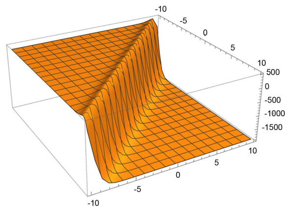
Figure 4. Simulation u_6(x,t) for Equation (12), with \alpha = 0.01 , \beta = -5 , \gamma = 3 , \kappa = 1 . The range of x and t are x \in [-10, 10] and t \in [-10, 10] . The jump appears in the middle.
