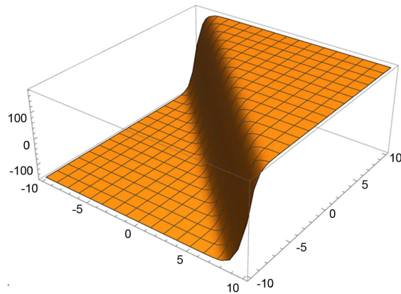
Figure 3. Simulation u_5(x,t) of Equation (11) with \alpha = 0.01 , \beta = -8 , \gamma = 3 , \kappa = 1 . The range of x and t are x \in [-10, 10] and t \in [-10, 10] . The jump appears in the middle.
