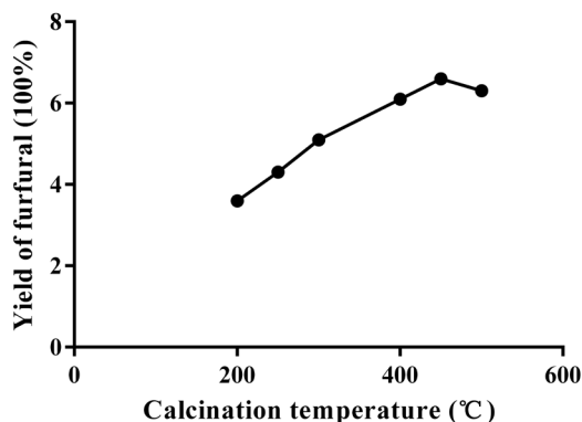
Figure 6. Effects of calcination temperature on yields of furfural preparation from nut shells Camellia oleifera Abel. Notes: The reaction conditions: concentration of sulfuric acid 1.1 mol/L, impregnation time 8 h, calcination time 4 h; hydrolysis of dose of catalyst 15 wt%, ratio of solid to liquid = 1:10 (g/ml), reaction temperature 100°C, reaction time 2 h.
