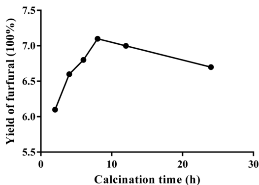
Figure 7. Effects of calcination time on yields of furfur preparation from nut shells Camellia oleifera Abel with sulfuric acid coating with niobic acid. Notes: The reaction conditions: concentration of sulfuric acid 1.1 mol/L, impregnation time 8 h, calcination temperature 450°C; Conditions of hydrolysis: dose of catalyst 15 wt%, ratio of solid to liquid = 1:10 (g/ml), reaction temperature 100°C, reaction time 2 h.
