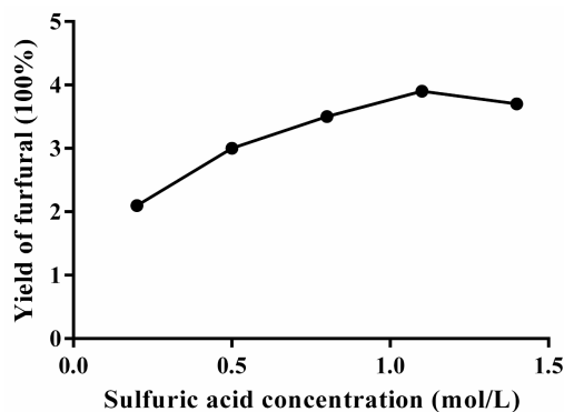
Figure 4. Effects of concentration of sulfuric acid on yields of furfural prepared from nut shell of camellia oleifera Abel. Note: impregnation time 4 h, calcination temperature 300°C, calcination time 4 h; The conditions of hydrolysis: dose of catalyst 15 wt%, ratio of solid to liquid = 1:10 (g/ml), reaction temperature 100°C, reaction time 2 h.
