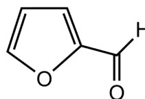
Furfural
