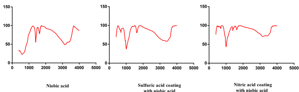
Figure 3. The spectra of FTIR of niobic acid and mineral acids coating with niobic acid. Notes: concentration of impregnated acids 0.8 mol/L, impregnation temperature 300°C, impregnation time 4 h; The conditions of hydrolysis: reaction temperature 100°C, ratio of solid to liquid = 1:10 (g/ml), dose of catalyst 15 wt%, reaction time 2 h.
