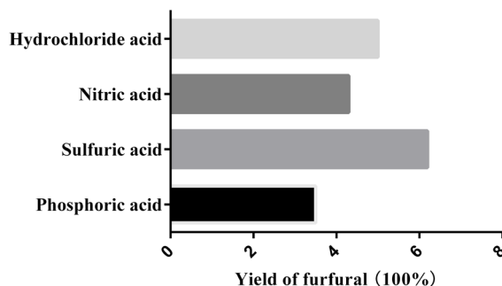
Figure 2. Yields of furfural from the nut shell of Camellia oleiferal Abel with mineral acids coating with niobic acid. Notes: concentration of impregnated acids 0.8 mol/L, impregnation temperature 300°C, impregnation time 4 h; The conditions of hydrolysis: dose of catalyst 15 wt%, ratio of solid to liquid = 1:10 (g/ml), reaction temperature 100°C, reaction time 2 h.
