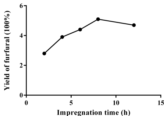
Figure 5. Effects of impregnation time on yields of furfural prepared from nut shell of Camellia oleifera Abel of sulfuric acid on niobic acid. Notes: The reaction conditions: concentration of sulfuric acid 1.1 mol/L, calcination temperature 300°C, calcination time 4 h; Conditions of hydrolysis: dose of catalyst 15 wt%, ratio of solid to liquid = 1:10 (g/ml), reaction temperature 100°C, reaction time 2 h.
