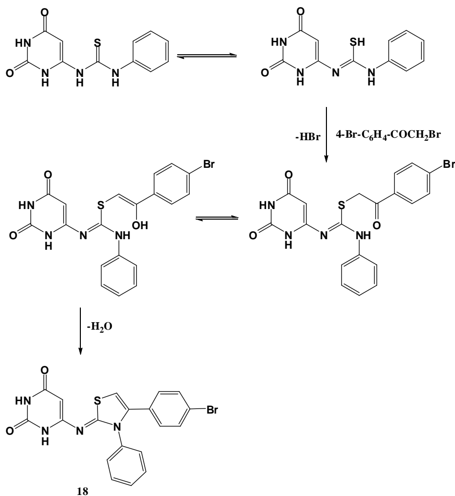
Figure 3. Reaction mechanism for the synthetic route for compound 18 .
