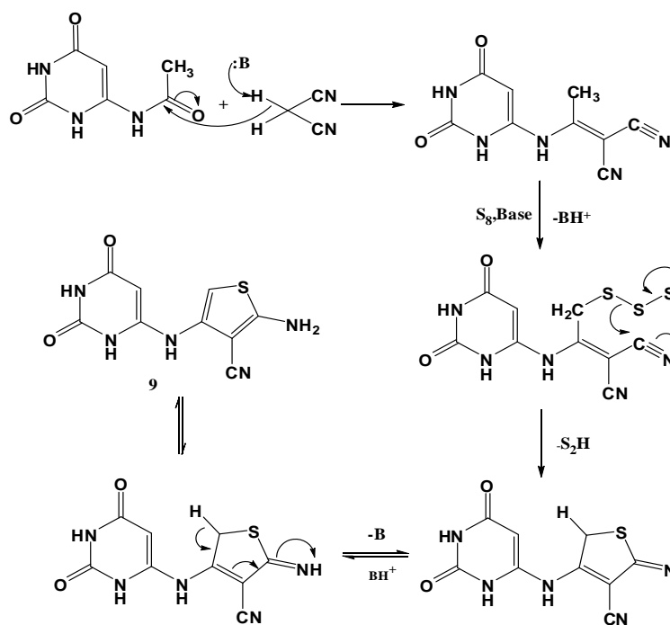
Figure 1. Reaction mechanism for the synthetic route of compound 9.
