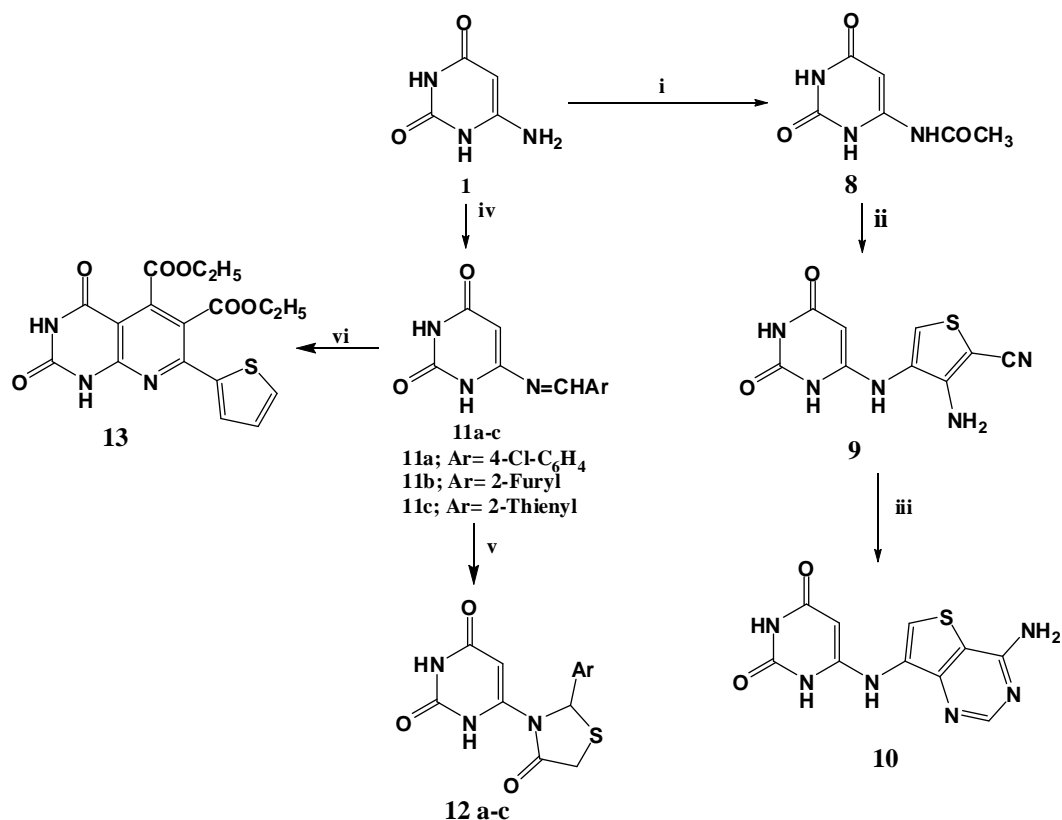
Scheme 2. Synthetic pathways for compounds 8 , 9 , 10 , 11a-c , 12a-c , and 13 . Reagents & conditions: i: (CH 3 CO) 2 O/gl.CH 3 COOH/steam bath; ii: malononitrile/sulphur/DMF/Reflux; iii: HCONH 2 /Reflux; iv: Ar-CHO/K 2 CO 3 /DMF/Reflux; v: HSCH 2 COOH/ZnCl 2 /Benzene/Reflux; vi: diethyl acetylene dicarboxylate/ Fusion.
