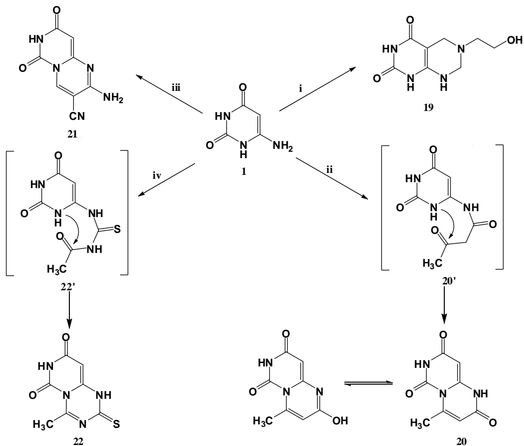
Scheme 4. Synthetic pathways for compounds 19, 20, 21 and 22. Reagents & conditions: i: \text{H}_2\text{NCH}_2\text{CH}_2\text{OH}/\text{HCHO}/\text{Abs. ethanol}/\text{Reflux} ; ii: \text{CH}_3\text{COCH}_2\text{COOC}_2\text{H}_5/\text{fusion} ; iii: \text{Ethoxymethylene malononitrile}/\text{piperidine}/\text{Abs. ethanol}/\text{Reflux} ; iv: \text{CH}_3\text{COCl}/\text{NH}_4\text{SCN}/\text{Acetone}/\text{Reflux} .
