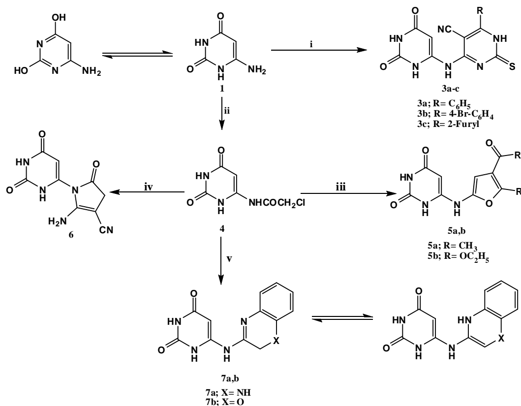
Scheme 1. Synthetic pathways for compounds 3a-c , 4 , 5 , 6 and 7a, b . Reagents & conditions: i: 4-Chlorodihydropyrimidine derivatives 2a-c /DMF/piperidine/Reflux; ii: ClCH 2 COCl/K 2 CO 3 /DMF/R.T.; iii: acetyl acetone or diethyl malonate/sod. ethoxide/Abs.ethanol/R.T.; iv: malononitrile/fusion; v: o-phenylene diamine or o-aminophenol/Abs. ethanol/TEA/Reflux.
