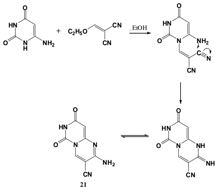
Figure 4. Reaction mechanism for the synthetic route for compound 21.
