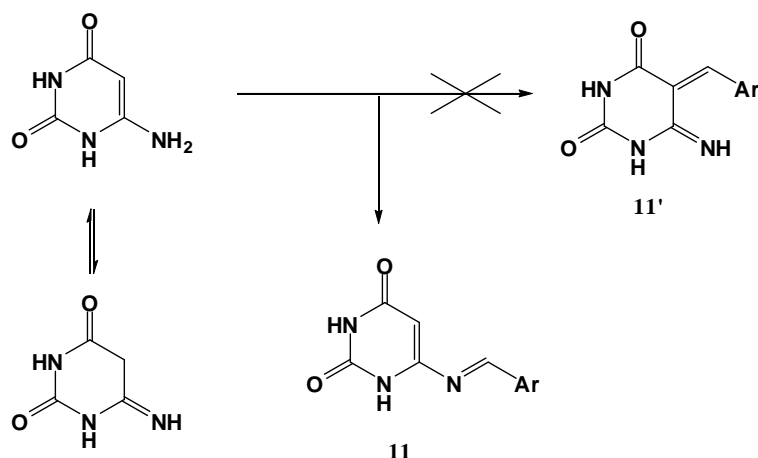
Figure 2. Possible reaction products of compound 11.
