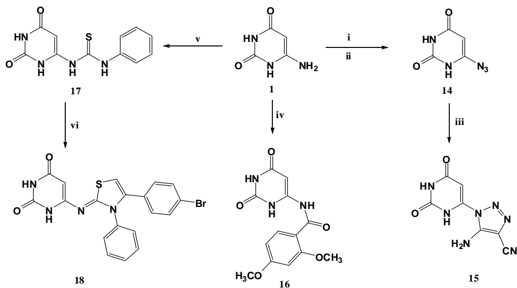
Scheme 3. Synthetic pathways for compounds 14, 15, 16, 17 and 18. Reagents & conditions: i : \text{NaNO}_2/\text{HCl}/0^\circ\text{C} ; ii : \text{NaN}_3/0^\circ\text{C} ; iii : malononitrile/sod. ethoxide/Abs. ethanol/Reflux; iv : 2,4-di( \text{OCH}_3 ) _2\text{C}_6\text{H}_3\text{COCl} /piperidine/DMF/Reflux; v : \text{C}_6\text{H}_5\text{NCS} /pyridine/Reflux; vi : 4-bromophenacyl bromide/Na acetate/Abs. ethanol/Reflux.
