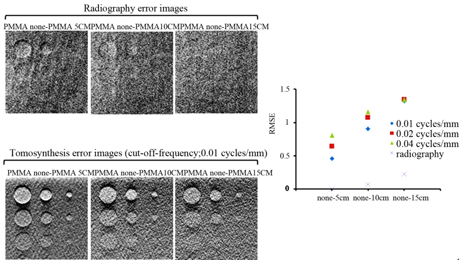
Figure 6. Comparison of RMSE with error images obtained from dual-energy subtraction digital tomosynthesis of different reconstruction kernels and the in-focus plane and dual-energy subtraction digital radiography.
