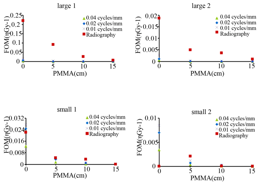
Figure 5. Effect of a dual-energy subtraction tomosynthesis of different reconstruction kernels and dual-energy subtraction digital radiography on FOM. A dual-energy subtraction digital tomosynthesis can confirm that the FOM value increases without direct exposure to large-size CaCO 3 content.
