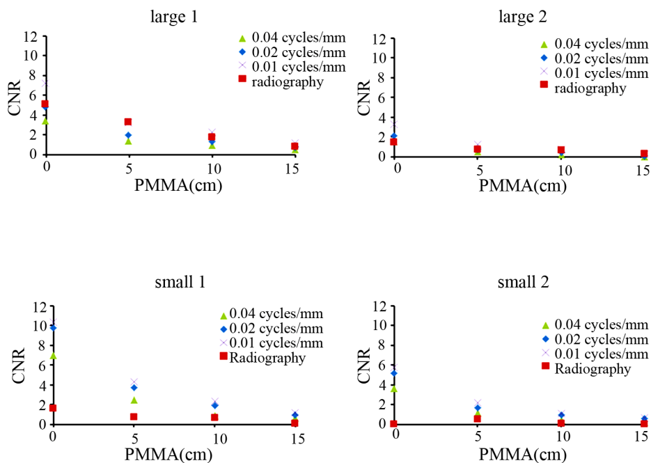
Figure 4. Effect of a dual-energy subtraction tomosynthesis of different reconstruction kernels and dual-energy subtraction digital radiography on CNR. A dual-energy subtraction digital tomosynthesis can confirm that the CNR value increases without direct exposure to large-size CaCO 3 content.
