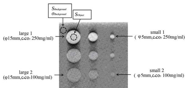
Figure 2. X-ray exposure acquisition setting for a single projection of the detectability phantom Areas of measurement for the evaluation and four analysis object metrics (large 1, large 2, small 1, and small 2) are shown.
