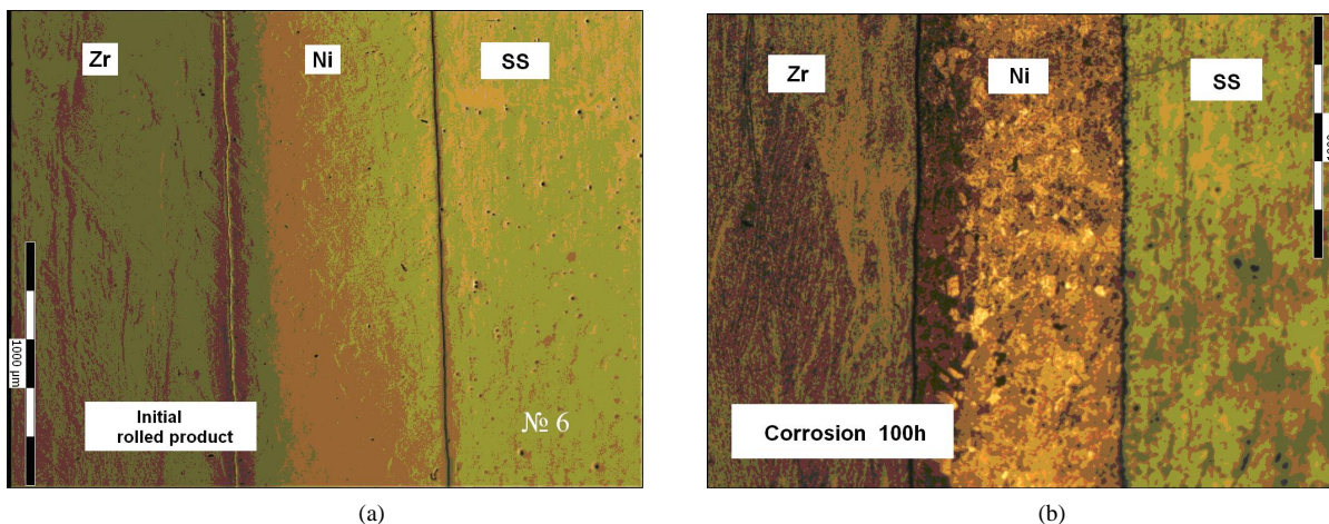
Figure 4. State of the surface of the solid-phase bonding Zr1Nb-Ni-SS: (a) In initial state; (b) After corrosion treatment during 100 hours.
