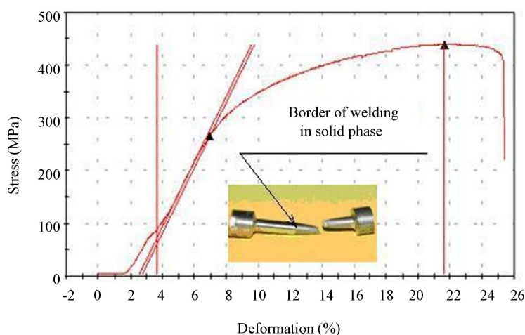
Figure 3. Tensile stress-deformation diagram of SS-C22E sample at 20°C. The inset below shows the point of specimen fracture in steel C22E.
