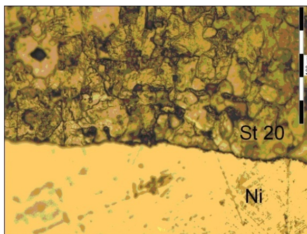
Figure 9. Microstructure of the solid-phase bonding C22E-Ni-SS on interface steel C22E -Ni after annealing at 500°C, 10 h (×200).
