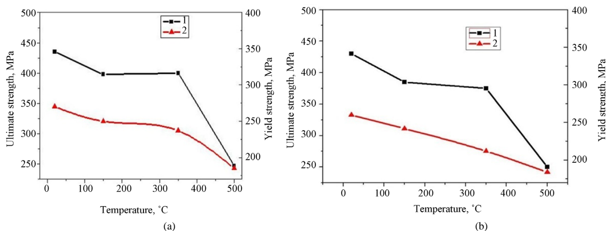
Figure 7. Temperature dependencies of mechanical characteristics of the solid-phase bonding steel C22E-SS (a) and steel C22E-Ni-SS (b); 1— \sigma_b ; 2— \sigma_{0.2} .
