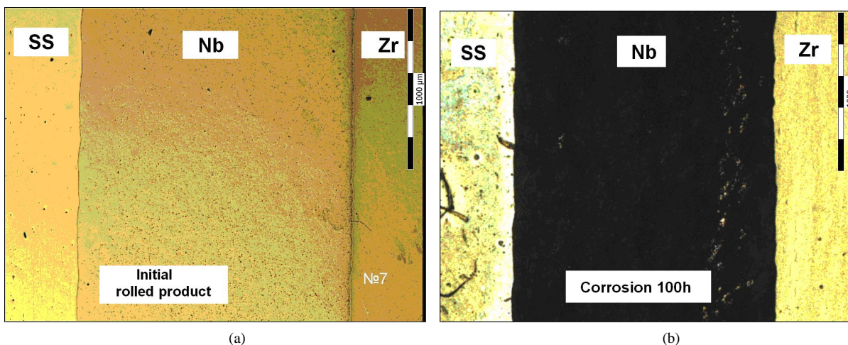
Figure 5. State of the surface of the solid-phase bonding Zr1Nb-Nb-SS: (a) In the initial state; (b) After corrosion treatment during 100 hours.
