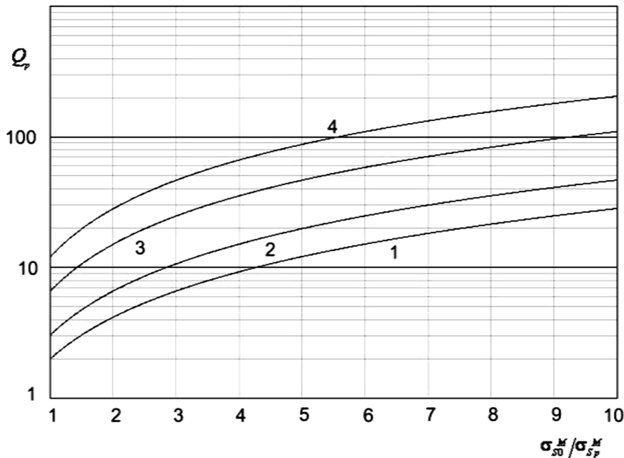
Figure 2. Dependence of relative strength coefficient of interface of joined metals on ratio of their yield strength \sigma_{S_0}^M / \sigma_{S_p}^M at different coefficients of yield strength range expansion: g = 1 (1); g = 1.5 (2); g = 3 (3); g = 5 (4).
