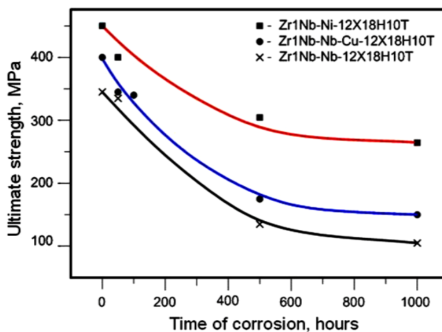
Figure 6. Dependence of ultimate strength of investigated composition on time of corrosion testing.
