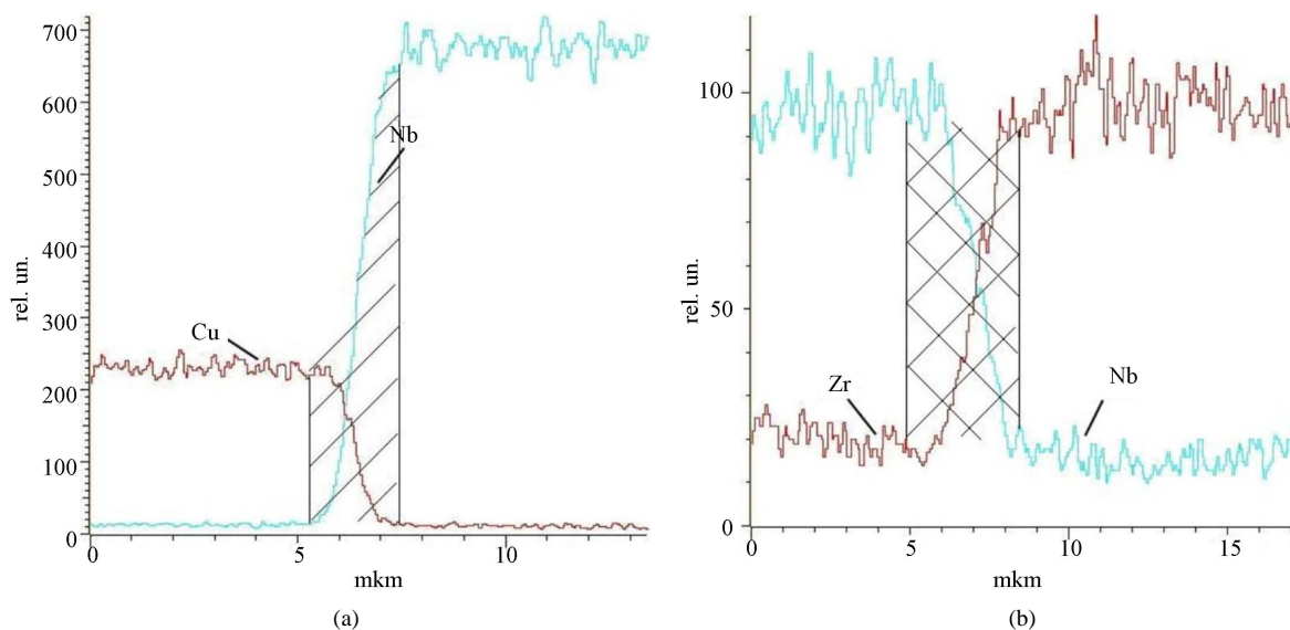
Figure 1. Spectra of micro X-ray spectrometric analysis near the interface of adjoint: (a) Niobium-copper; (b) Niobium-zirconium.
