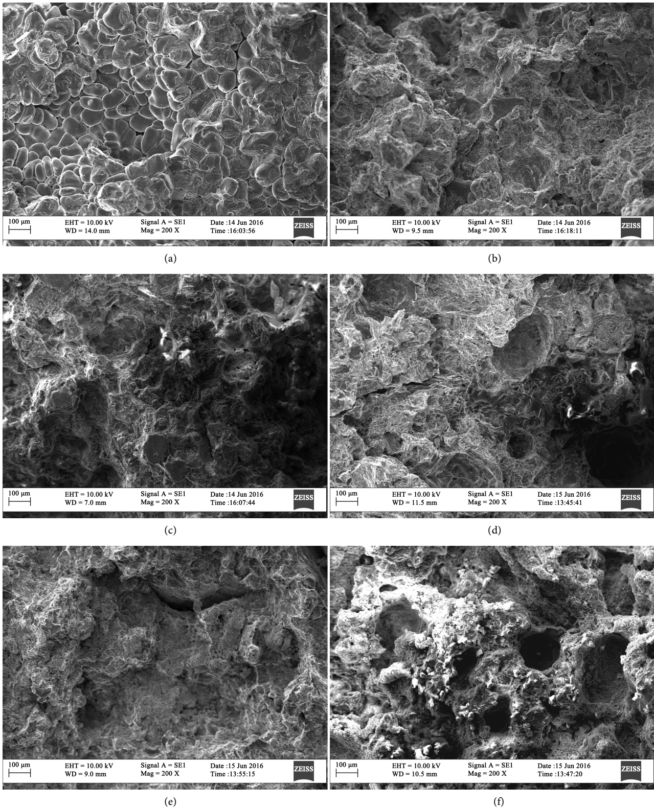
Figure 7. SEM images of fractured surfaces of (a) 0 wt%; (b) 2 wt%; (c) 4 wt%; (d) 6 wt%; (e) 8 wt%; (f) 10 wt% at 200 \times .
