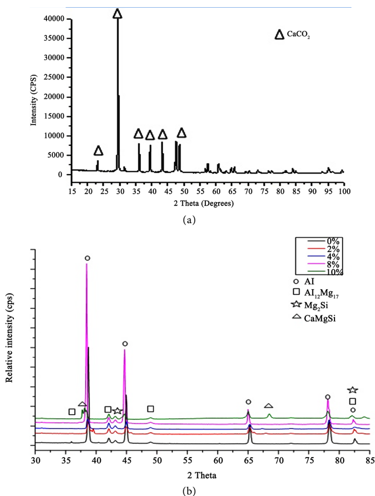
Figure 4. (a) XRD pattern of eggshell (ES); (b) XRD pattern of composites.
