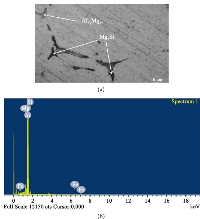
Figure 2. (a) Optical micrograph and (b) EDX spectra of as-cast Al6061 matrix alloy.
