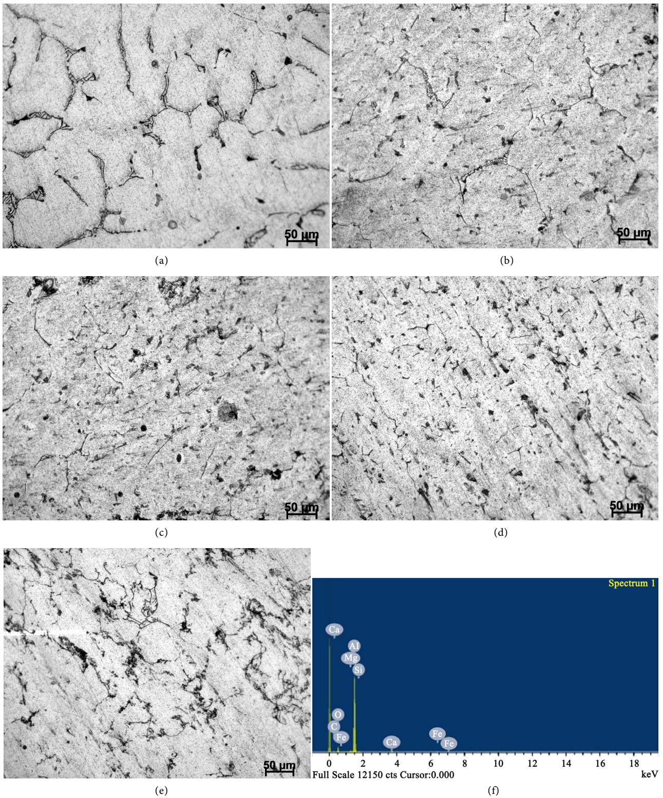
Figure 3. Optical micrographs ES-reinforced Al6061 alloy matrix composites: (a) 2 wt%; (b) 4 wt%; (c) 6 wt%; (d) 8 wt%; (e) 10 wt% of ES and (f) EDS spectra of 4 wt% composite.
