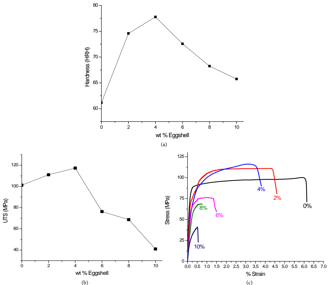
Figure 6. (a) Hardness variation of composites; (b) Tensile strength variation of composites; (c) Stress-strain curves of unreinforced and reinforced composites.
