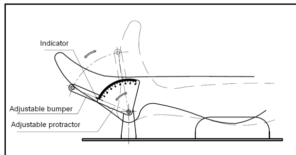
Figure 4. The goniometer. Measurement of the passive range of motion of plantar and dorsiflexion. The term “passive range of motion” refers to the radius of motion achieved by external force without using the patient’s own muscles.
