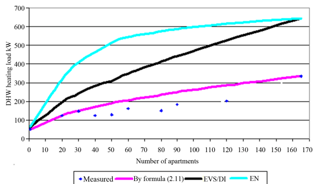
Figure 5. DHW design heating load depending on the number of apartments by the EVS (D1) standard, the EN standard and the proposed formula together with the points calculated on the basis of the results of measuring.
