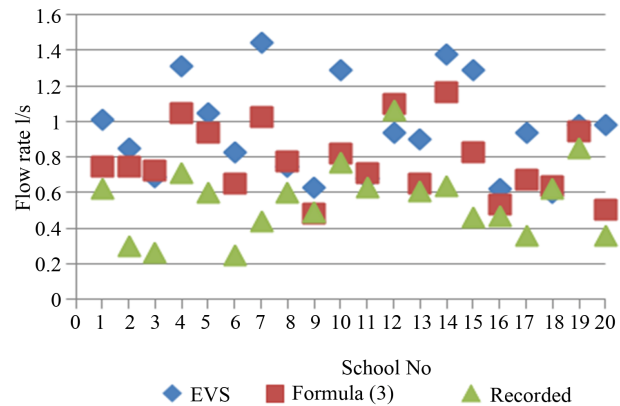
Figure 6. Comparison of the design flow rates determined for schools by the empiric Formula (3), the standard EVS 835 and recorded values.
