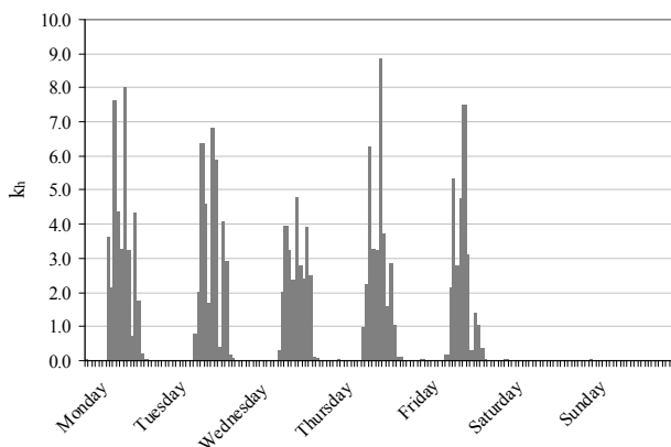
Figure 8. Weekly variability graph of DHW consumption in kindergarten.
