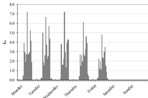
Figure 10. Weekly variability graph of DHW consumption in office building.
