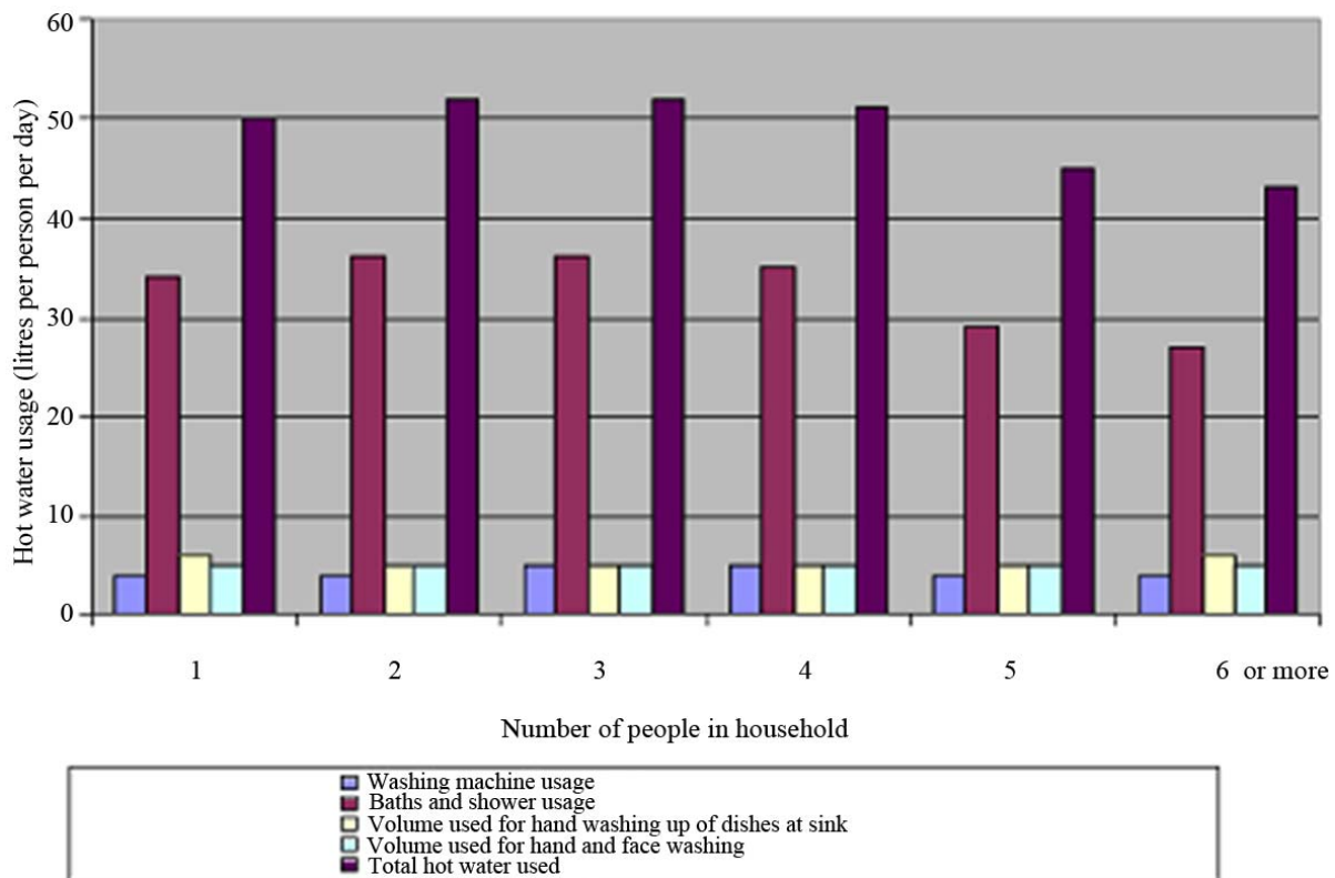
Figure 1. Average DHW consumption depending on the number of inhabitants in the households.
