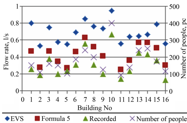
Figure 9. Comparison of the design flow rates determined for office buildings by the empiric formula (5), the standard EVS 835 and recorded values.
