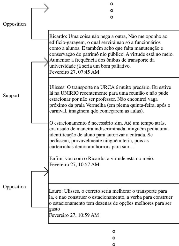
Figure 4. Discourse analysis.
