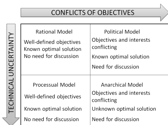
Figure 1. Discussion models [3].
