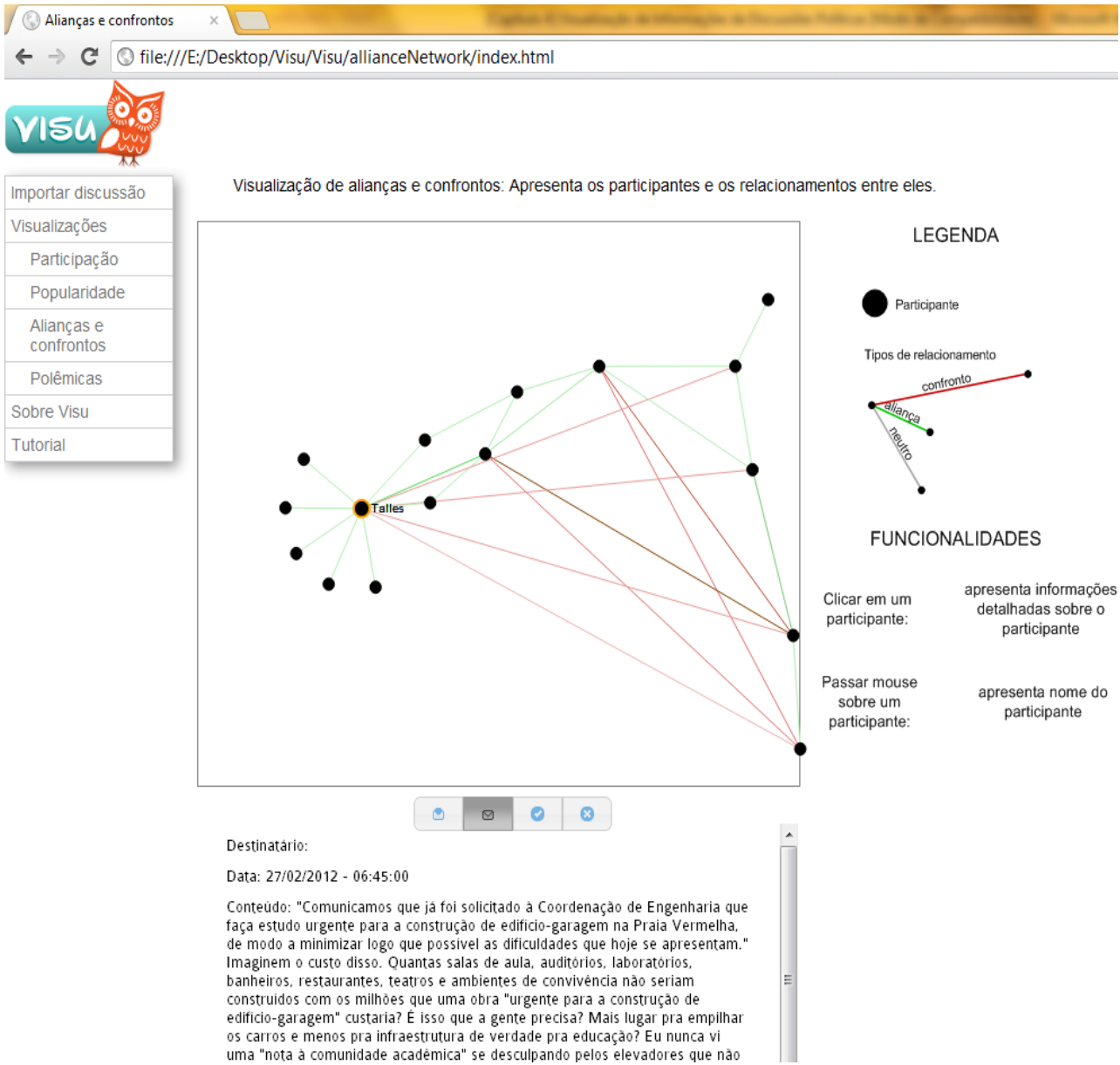
Figure 7. Final network and interactions in Visu.
