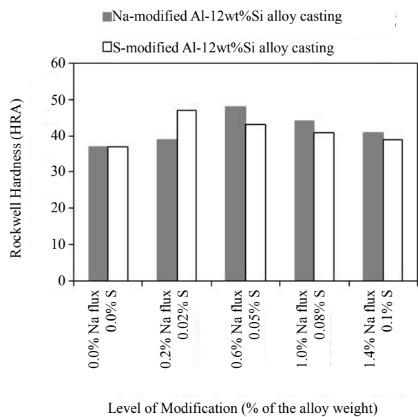
Figure 13. Effect of modification level on the hardness of Al-12wt%Si alloy casting.
