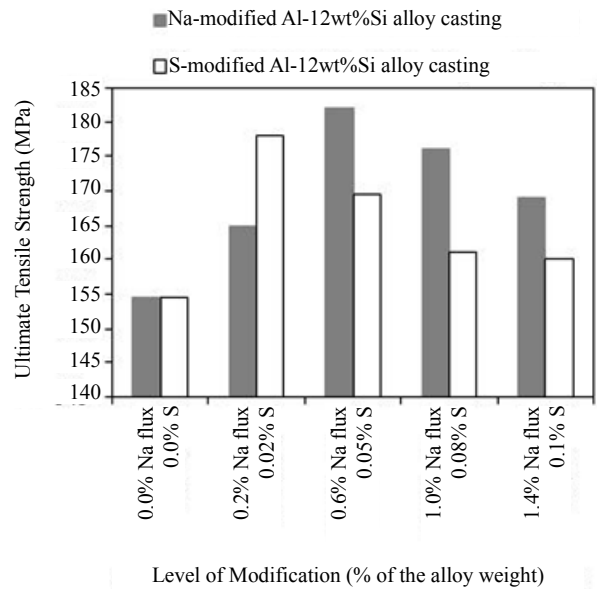
Figure 10. Effect of modification level on the ultimate tensile strength of Al-12wt%Si alloy casting.
