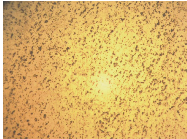
Figure 6. Micrograph of Al-12wt%Si + 1.0% Na flux alloy casting (400 \times ).
