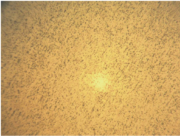
Figure 4. Micrograph of Al-12wt%Si + 0.6% Na flux alloy casting (200 \times ).
