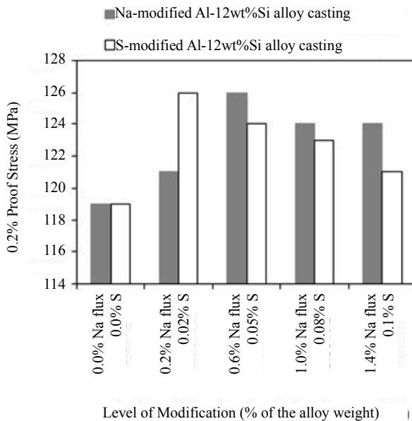
Figure 11. Effect of modification level on the 0.2% proof stress of Al-12wt%Si alloy casting.
