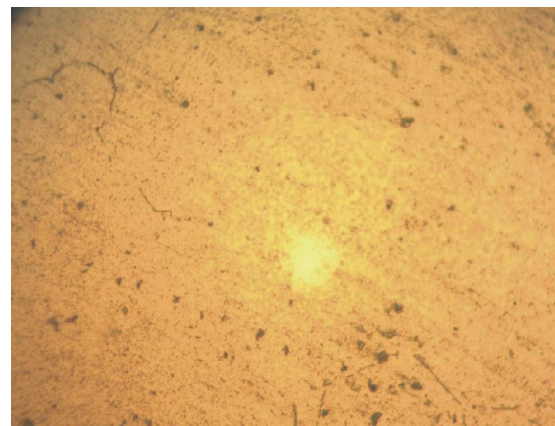
Figure 3. Micrograph of Al-12wt%Si + 0.02% S alloy casting (200×).
