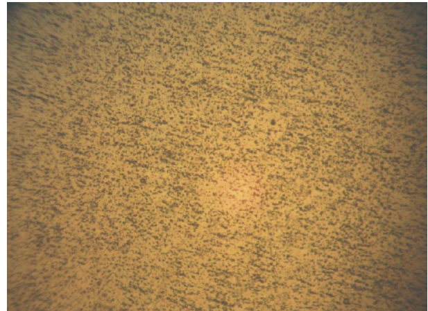
Figure 7. Micrograph of Al-12wt%Si + 0.08% S alloy casting (200 \times ).
