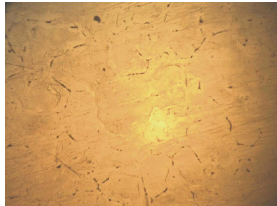
Figure 2. Micrograph of Al-12wt%Si + 0.2% Na flux alloy casting (200×).
