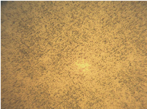
Figure 5. Micrograph of Al-12wt%Si + 0.05% S alloy casting (200 \times ).
