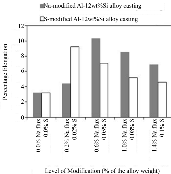
Figure 12. Effect of modification level on the percentage elongation of Al-12wt%Si alloy casting.
