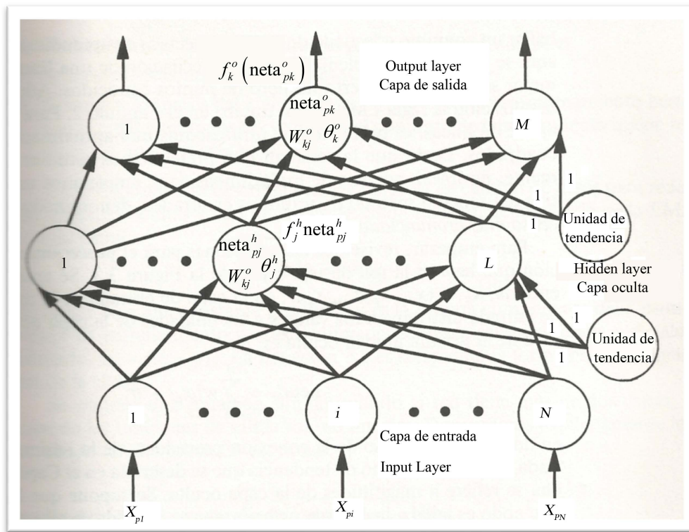
Figure 3. Typical layout of a Feedforward-type neural network.
