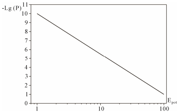
Figure 3. Probability of the severe accident as a function of potential energy stored in RF coolant ( E_{pot} , MJ/m 3 ).
