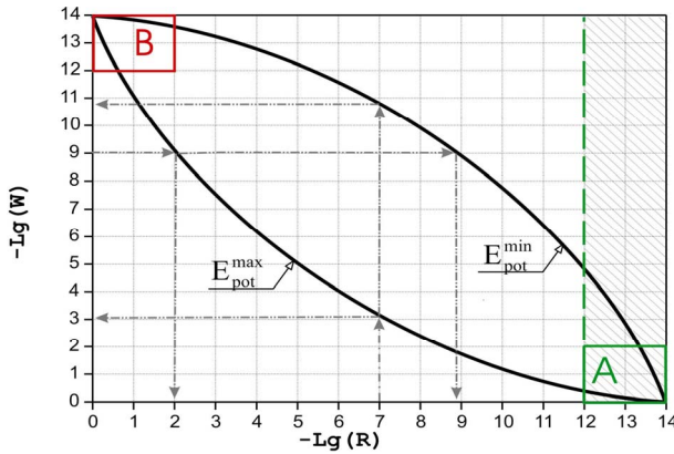
Figure 1. Safety diagram.
