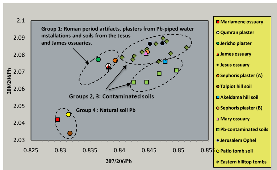
Figure 6. Plot of the isotopes ^{208/206}\text{Pb} vs. ^{207/206}\text{Pb} . Group 1 contains the isotope values for the James and Jesus ossuaries and plasters from Roman period water installations. Group 2 encloses values for soils from the EHT ossuaries, the Mary, one Sepphoris and two Ancient Jerusalem (Ophel) water installations. Group 3 contains values for contaminated soils and Group 4 values for soils from the Mariamene ossuary, Patio tomb and Talpiot hill.
