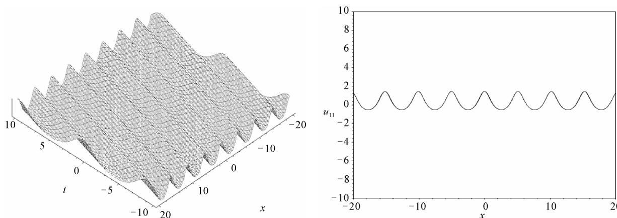
Figure 2. The plot of the periodic traveling wave solution u_{11} to (1.1) with c_2 = 0.5, k_1 = 0.9 and the initial status of u_{11} .
