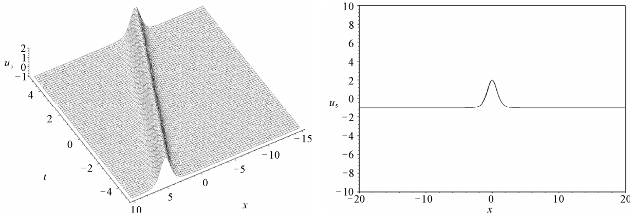
Figure 1. The plot of the peak-shaped solitary wave solution u_5 to (1.1) with c_2 = 1 and the initial status of u_5 .
