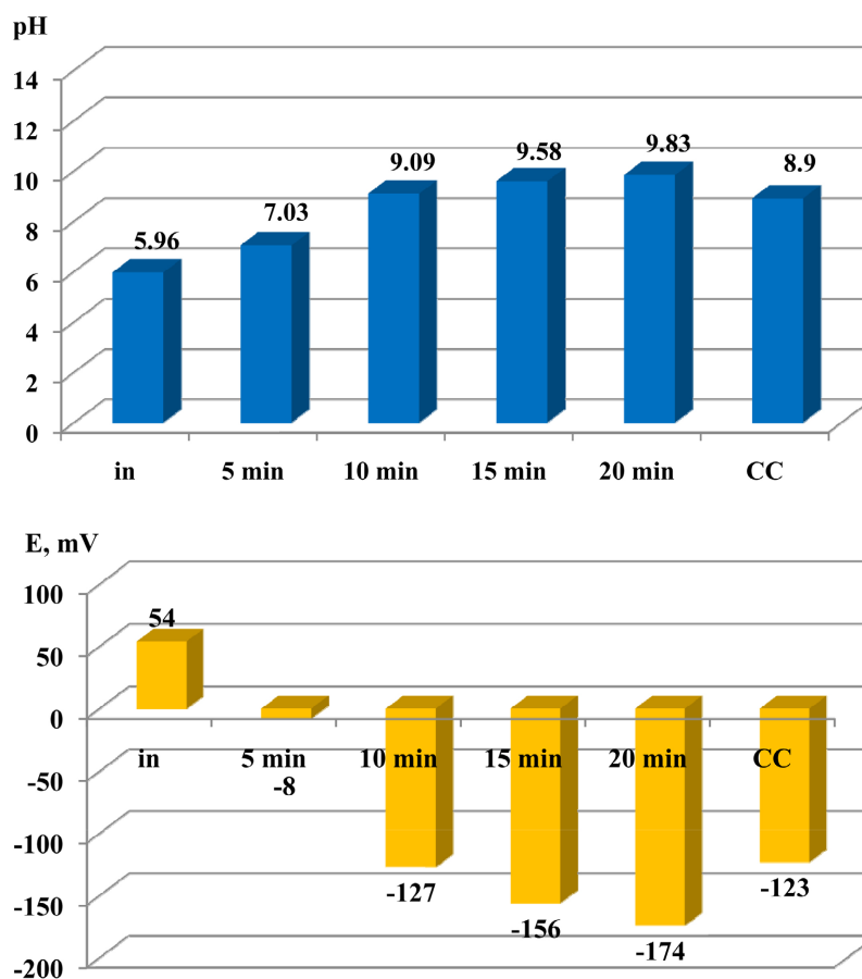
Figure 6. Variation of pH and redox potential (E, mV) values at 1:3 diluted RBY electroactivation (C2). j = 20 \text{ mA/cm}^2 ; CC S—Cathode cell content (foam phase); CC L—Cathode cell content (liquid phase).
