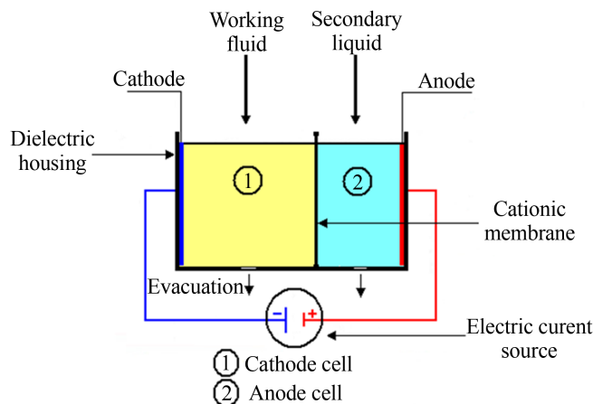
Figure 2. Scheme of the EDP-0.5 diaphragm electrolyzer.
