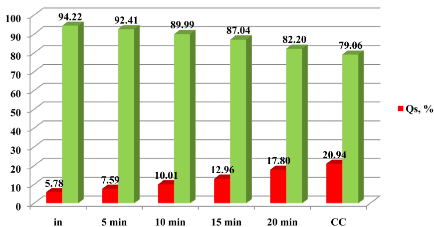
Figure 7. Variation of protein content upon electroactivation of diluted RBY (1:5). j = 20 \text{ mA/cm}^2 (C3); protein content: PCRBY (Qp, %) and HPRBY (Qs, %).
