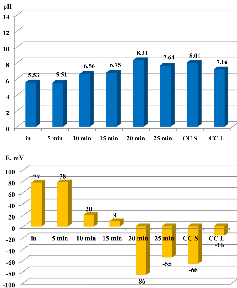
Figure 4. Variation of pH values and redox potential ( E , mV) when electroactivating undiluted RBY (C1). j = 20 \text{ mA/cm}^2 ; CC S—Cathode cell content (foam phase); CC L—Cathode cell content (liquid phase).
