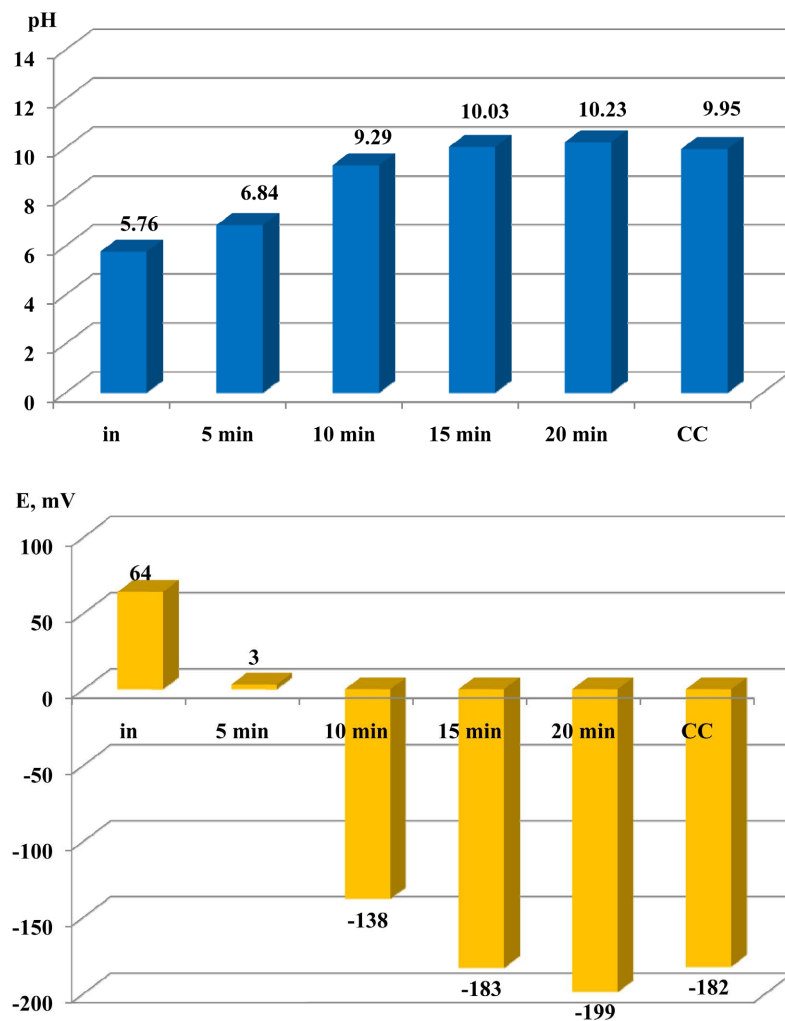
Figure 8. Variation of pH and redox potential (E, mV) values at 1:5 diluted RBY electroactivation (C3). j = 20 \text{ mA/cm}^2 .
