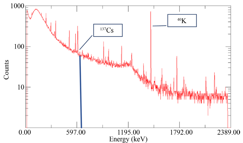
Figure 1. Spectrum of sample FM1 obtained with HPGe detector with marked 137 Cs photoppeak.
