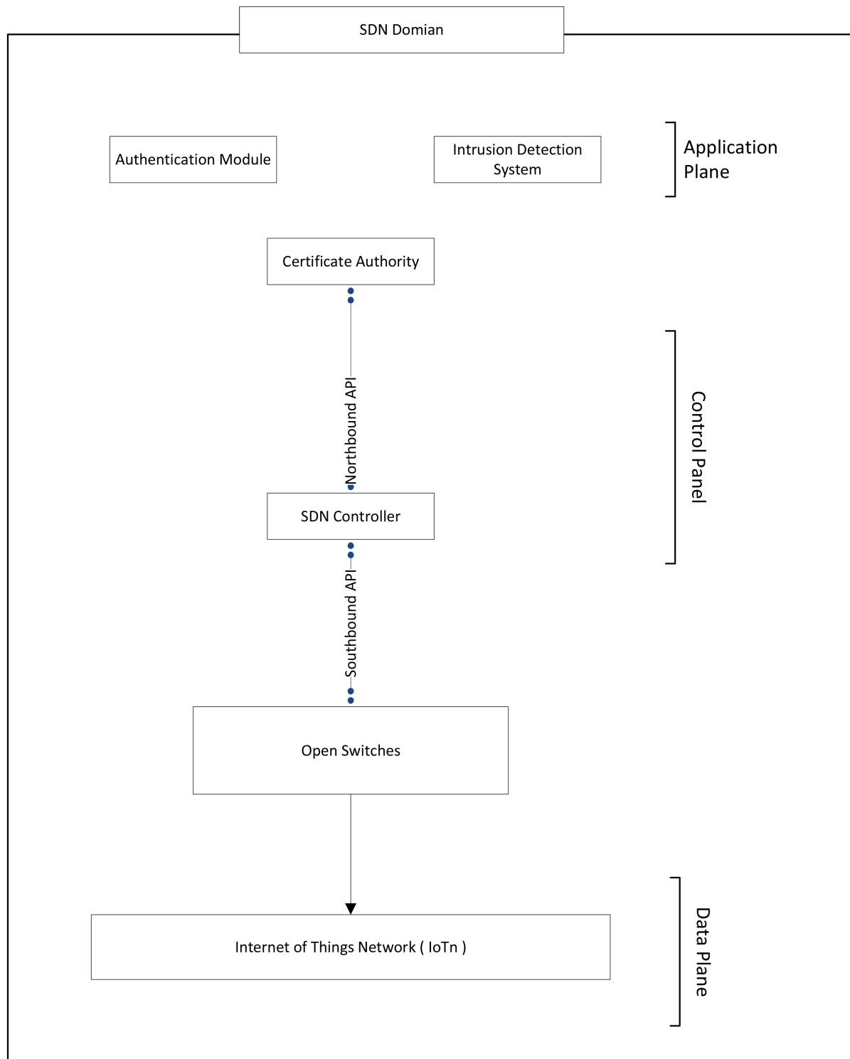
Figure 1. The architecture of the proposed model.
