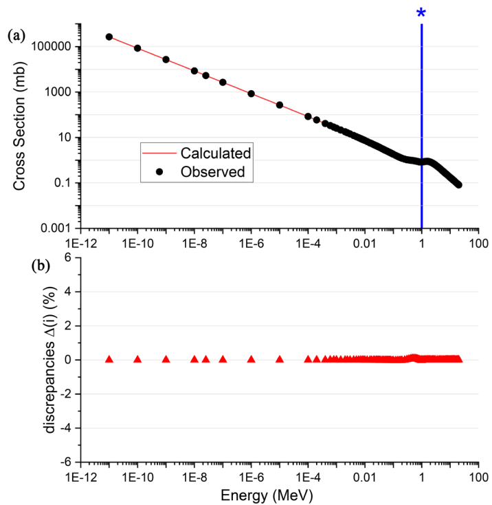
Figure 2. (a) Empirical formula of cross section of ^3\text{He} (n, p) ^3\text{H} Nuclear Reaction as a function of neutron incident energy. (b) Discrepancies between observed and calculated data. *Data before the line: E = 1 MeV are taken from Equation (12), while those after the line are taken from Equation (13).
