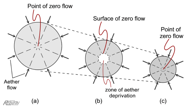
Figure 5. If the mass of a neutron star is greater than 3.4 Suns, then the excess mass will quickly be lost. The loss occurs during the gravitational collapse to the Terminal state. The mechanism involves the increase in density, (a) through (c). Simultaneously, the surface area decreases, thus critically reducing the supply of aether—essentially chocking off the flow to the core of the structure, (b). Mass vanishes within the “zone of aether deprivation,” as it has been labelled in part (b) and shown greatly exaggerated. Mass literally disappears from the Universe; the reason being that matter simply cannot exist without a sustained supply of the universal essence we call aether. The aether deprivation zone immediately collapses to a point at the heart of what is now the Terminal state structure, (c).
