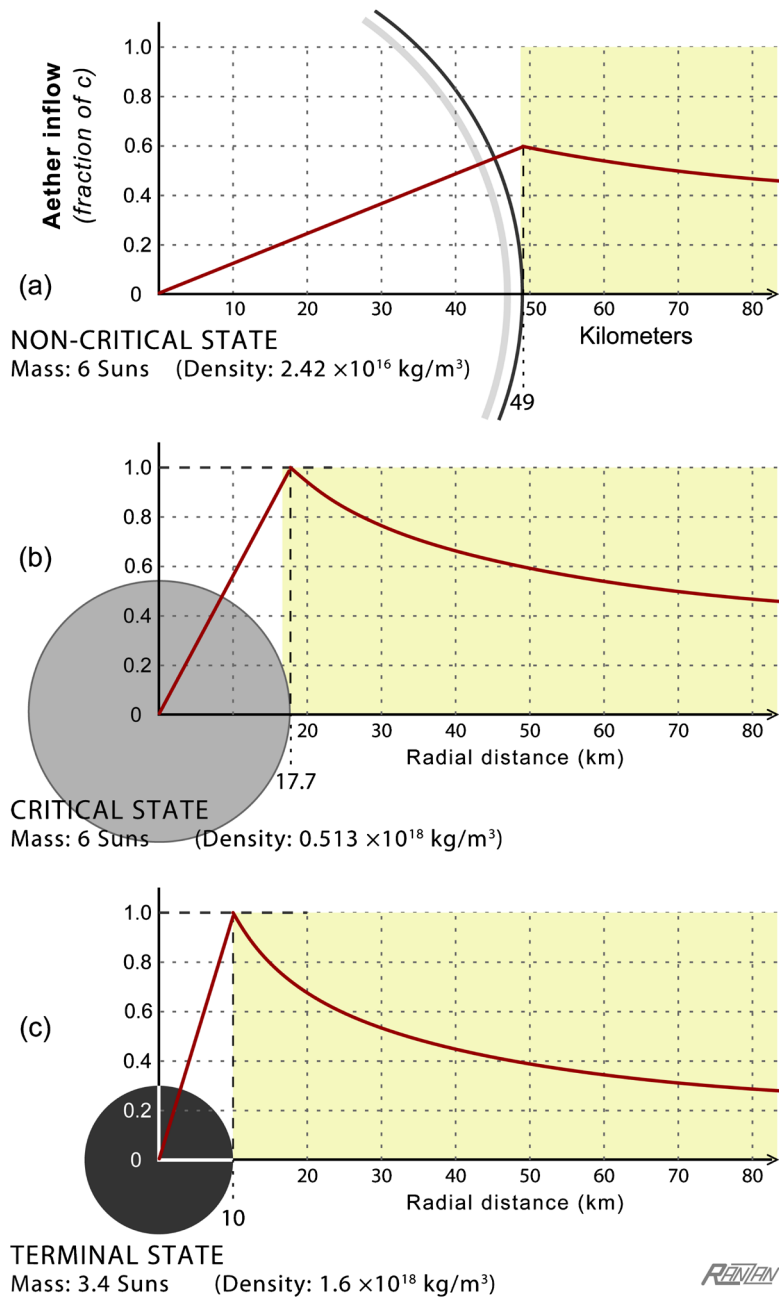
Figure 4. Gravitational contraction of a 6-solar-mass body. In snapshot (a) the structure is in the NON-CRITICAL state. At the instant represented here, the aether inflow (at the surface) is six-tenths lightspeed and the radius is 49 kilometers. Snapshot (b) shows the instant the structure, now shrunk to radius 17.7 kilometers, becomes CRITICAL. The collapse ends in snapshot (c) with the attainment of the ultimate density state—but with the loss of considerable mass! So, what happened to the missing mass?
