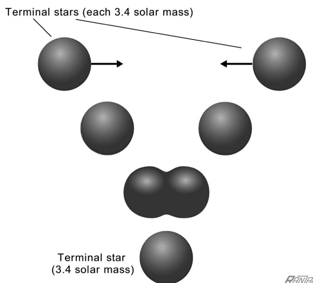
Figure 6. Merger of two Terminal stars. The result is a single Terminal star identical in size and mass to just one of the original. Only the rotation rate (and the orientation) is subject to change. Remarkably, the mass equivalence of 3.4 Suns completely vanishes and represents a local violation of the principle of matter conservation. (Polar jets are usually present, but are not shown.)
