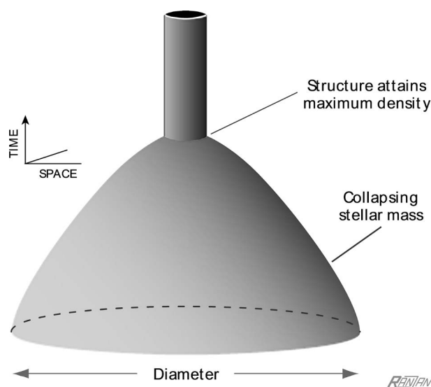
Figure 1. Gravitational collapse halts when mass concentration attains the ultimate density. Based on 1) the existence of aether, as was defined; 2) the innate absorption/consumption of aether by all matter; 3) the reasonable assumption of the existence of a density limit; and 4) the concentration or aggregation of sufficient degenerate mass having complete absence of thermal agitation; based on those factors, nature follows a course that ultimately leads to a final stage of gravitational collapse (shown in the schematic). The end result is a compact-and-stable structure with maximal density.
