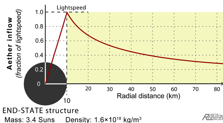
Figure 3. Anatomy of the end-state neutron star or, synonymously, the Terminal neutron star . Based on the assumption of ultimate density being 1.60 \times 10^{18} \text{ kg/m}^3 , the end-state structure necessarily has a total mass of 3.4M_{\odot} , a radius of 10 kilometers, a pure energy surface layer, and an aether inflow profile as shown. If the density-value assumption is off the true value, then it would simply change the diameter of the end-state structure.
