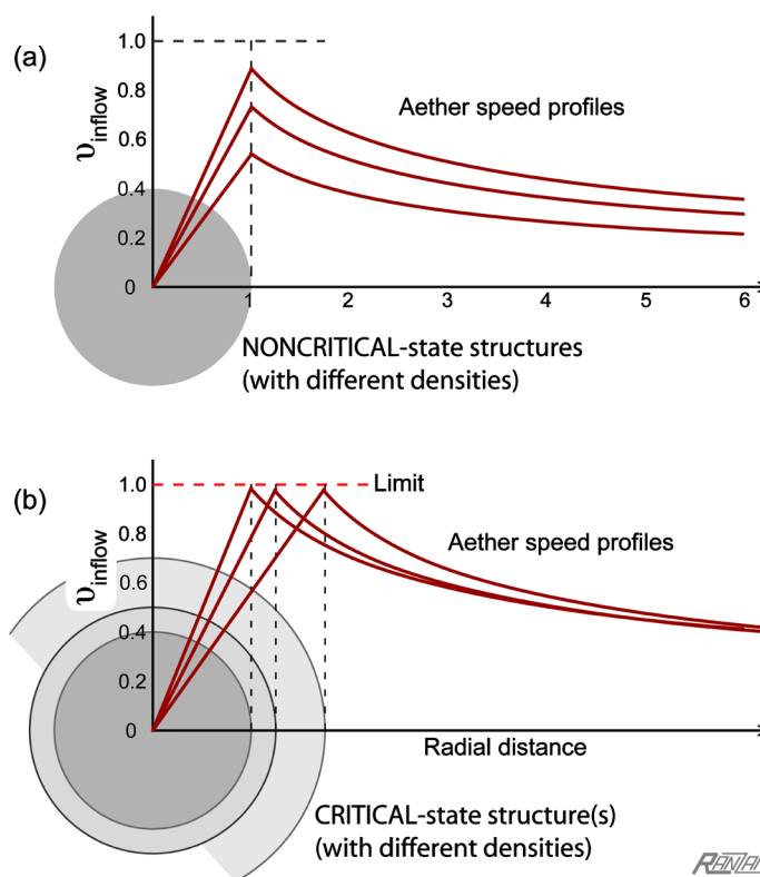
Figure 2. Aether inflow profiles relating to gravitational collapsed structures. Part (a) gives representative profiles of same-size structures but with different densities. Although they have undergone serious collapse, or contraction, they are clearly not in the critical state . Part (b) illustrates one of the two essential conditions for attaining the ultimate density of mass. Here is a structure that has contracted down to the critical state , as indicated by the fact that the profile touches the “lightspeed line”. As the collapse progresses in the manner shown here, the density increases—or at least that is the assumption being made. During the ongoing collapse process, there is really no way of knowing when the state of maximum possible density is reached. (The aether speed v_{\text{inflow}} is given as a fraction of lightspeed.)
