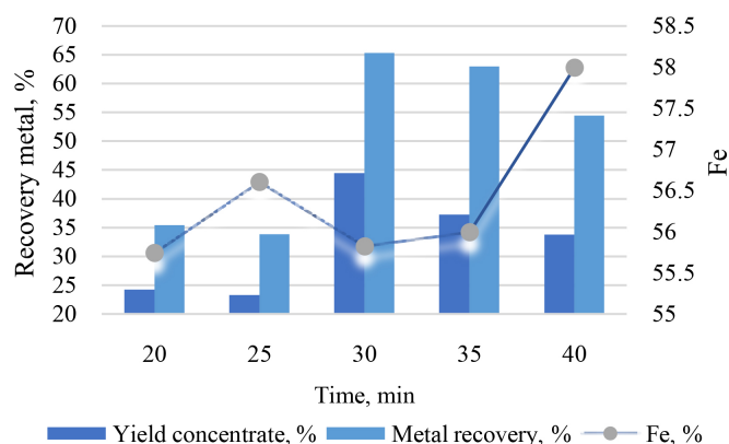
Figure 30. Wet magnetic beneficiation 4A.
