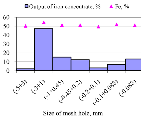
Figure 23. Grain size distribution curve.
