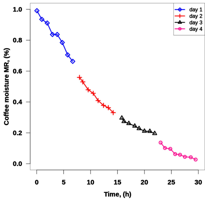
Figure 8. Variation of coffee moisture content with time during drying.
