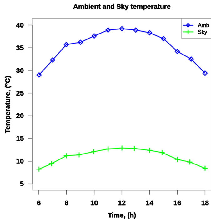
Figure 4. Temporal variation of ambient and sky temperatures.
