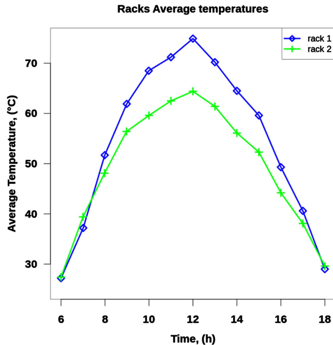
Figure 6. Average temperatures of the racks for three days.
