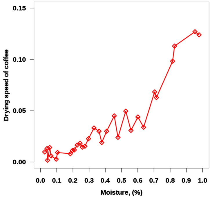
Figure 9. Variation in drying speed of coffee as a function of moisture content.
