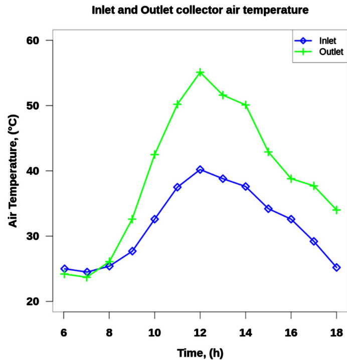
Figure 5. Evolution of air temperatures at the inlet and outlet of the collector.
