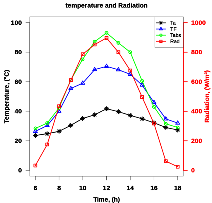
Figure 3. Curve of different temperatures at the sensor.
