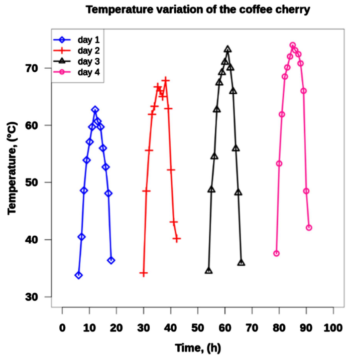
Figure 7. Temperature variation of the coffee cherry on the first rack.
