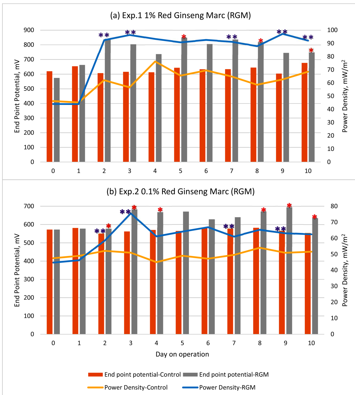
Figure 2. End point potential (bars; mV, open circuit voltage) and power density (lines; mW/m 2 ) in MFCs supplemented with 1% ((a) Exp. 1) or 0.1% ((b) Exp. 2) of red ginseng marc (RGM) during 10d operation. *Means of end point potential between control and RGM differ ( P < 0.05 ). **Means of power density between control and RGM differ ( P < 0.05 ).
