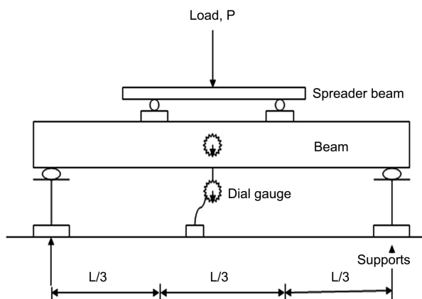
Figure 4. Test arrangements for determination of bending strength.
