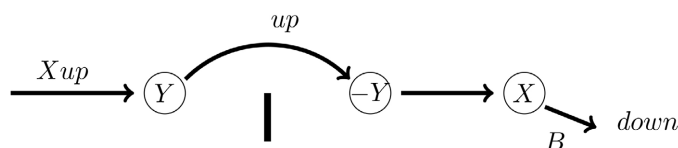
Figure 4. Train of Stern-Gerlach devices with blocking system.
