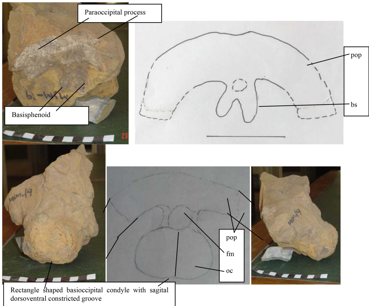
Figure 3. Gspisaurus pakistani holotypic braincase MSM-62-19 from Alam 19 in anterior, posterior and lateral views. Scale in image, each black or white digit is 1 cm. Scale bar in line drawing represents 5 cm. Abbreviations: bs, basisphenoid; oc, occipital condyle; fm, foramen magnum; pop, paraoccipital process; GSP, Geological Survey of Pakistan; MSM, Muhammad Sadiq Malkani. The formal specimen numbers are like GSP/MSM-62-19 but briefly represented by MSM-62-19 in literature. The central number 62 represents the serial number of specimen/fossil, and last number 19 represents locality number of Alam locality. Further at places the locality name with locality number are mentioned as like Alam 19, here Alam is the locality name and 19 is the locality number. At places 19 or 19c which means central Alam, the south Alam is represented by 19s and north Alam is represented by 19n.
