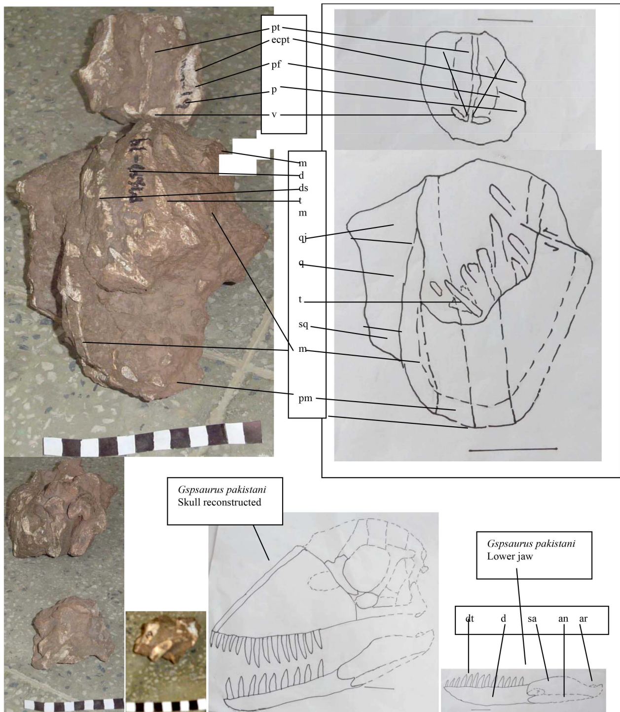
Figure 2. Gspisaurus pakistani holotypic skulls MSM-79-19 (larger specimen) and MSM-80-19 (smaller specimen) found from Alam locality. Skull and mandible reconstruction after fossils and estimation. Scale in image, each black or white digit is 1 cm. Scale bar in line drawing represents 5 cm. Abbreviations: d, dentary; dr, dentary ramus; ds, dentary symphysis; ecpt, ectopterygoid; ml, midline contact; m, maxilla; mr, maxillary ramus; p, palatine; ph, palatal dorsal hook; pt, pterygoid; q, quadrate; gj, quadratojugal; sq, squamosal; t, teeth; v, vomerine.
