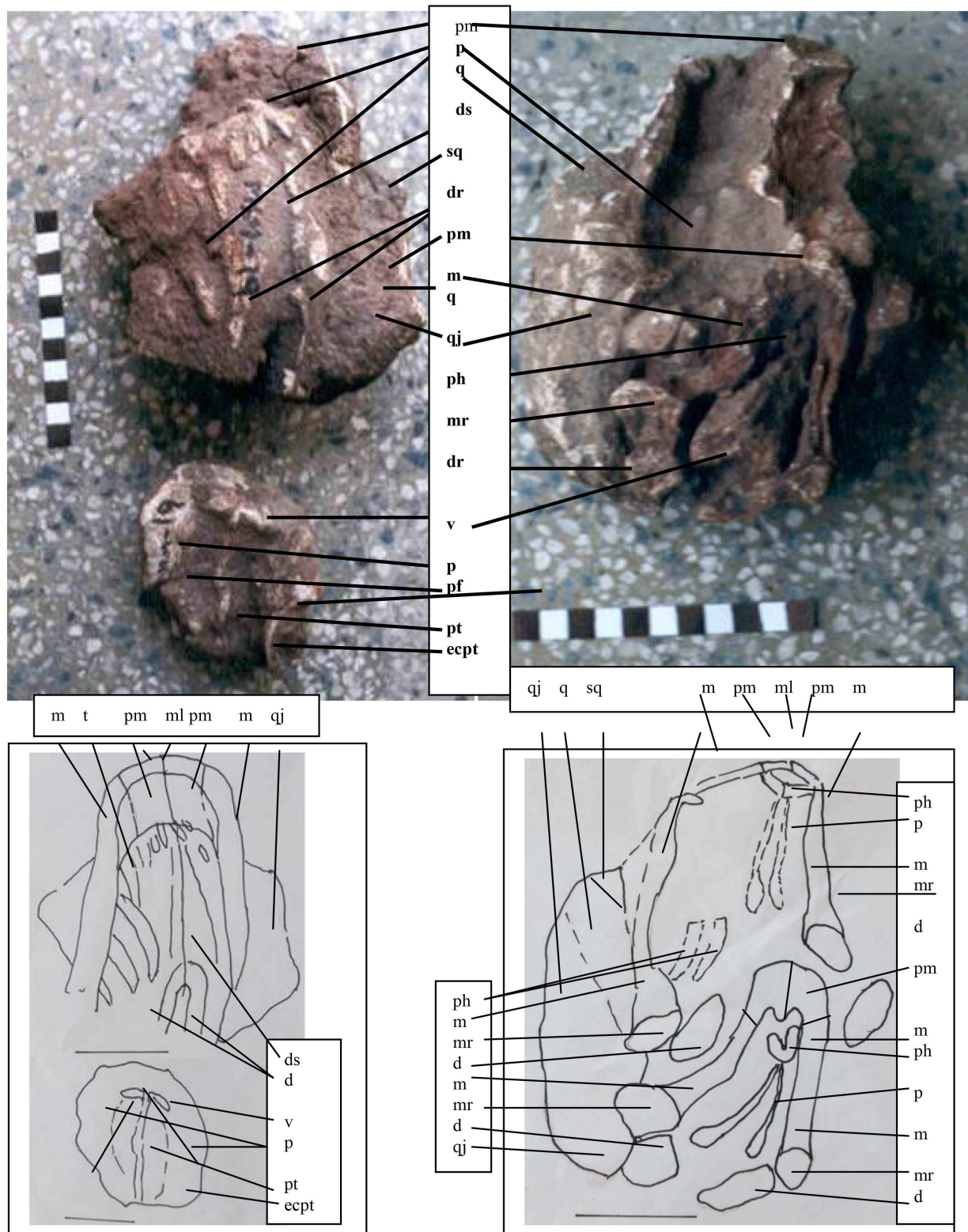
Figure 1. Images and line drawings of Gpsaurus pakistani holotypic skull MSM-79-19 and MSM-80-19 in ventral and posterior cross sectional views. Scale, each black/white digit is 1 cm. Scale bar in line drawing represents 5 cm. Abbreviations: d, dentary; dr, dentary ramus; ds, dentary symphysis; ecpt, ectopterygoid; ml, midline contact; m, maxilla; mr, maxillary ramus; p, palatine; ph, palatal dorsal hook; pt, pterygoid; q, quadrate; gj, quadratojugal; sq, squamosal; t, teeth; v, vomerine. Gpsaurus pakistani includes holotype in Figures 1-4 .
