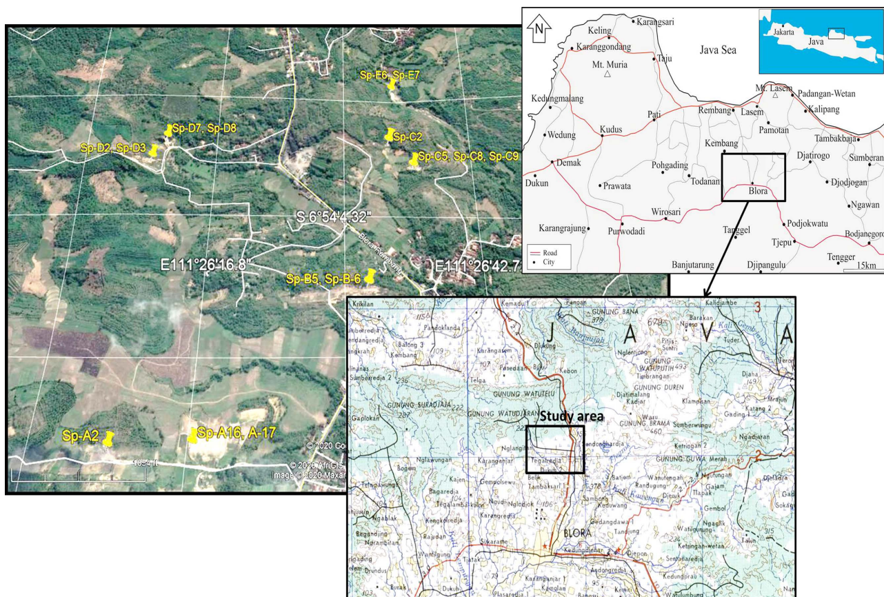
Figure 1. Location map of Rembang area in Northeast Java, Indonesia.
