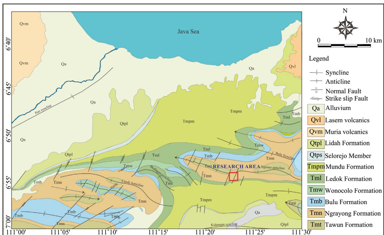
Figure 2. Regional geological map of Rembang area and surrounding area, Northeast Java, Indonesia [20].
