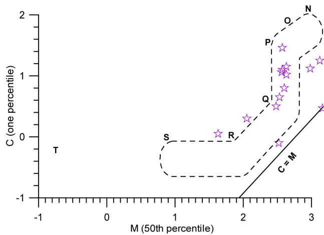
Figure 9. C-M plot showing the transporting mechanism of Ngrayong Sandstones. Rolling (ON); rolling and suspension (PO); suspension and rolling (QP): graded suspension, mainly saltation (QR); uniform suspension (SR); pelagic suspension (T).
