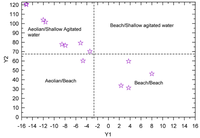
Figure 7. Cross plots of the linear discriminant functions (Y1 vs. Y2) of the Ngrayong sediments.
