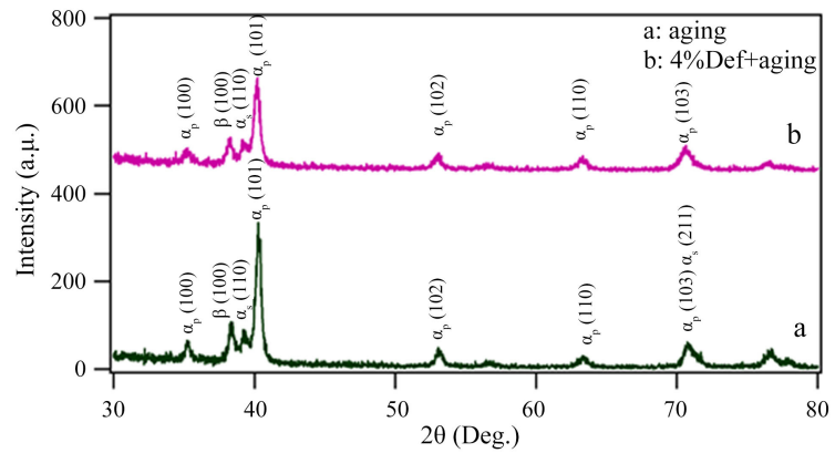
Figure 3. XRD pattern of aging only and 4% Def + aging conditions.
