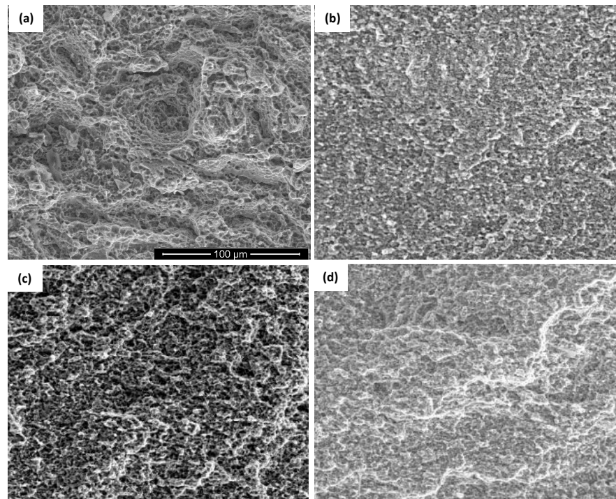
Figure 7. Fracture surface of tensile samples (a) swaged, (b) aging only, (c) 2% Def + aging and (d) 4% Def + aging.
