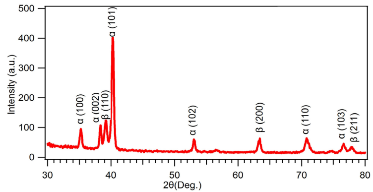
Figure 2. XRD pattern of the as-cast TC21 Ti-alloy.
