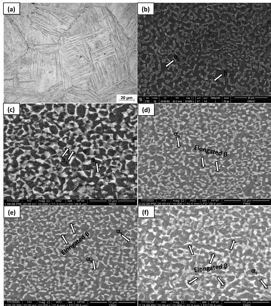
Figure 1. FESEM micrographs showing the microstructures of conditions (a) as-cast, (b) swaged, (c) aging only, (d) 2% Def + aging, (e) 3% Def + aging and (f) 4% Def + aging, samples of TC21Ti-alloy.
