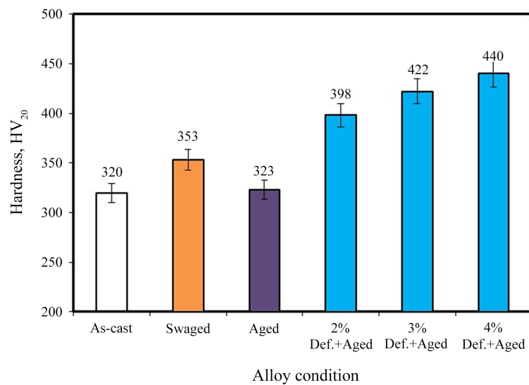
Figure 4. Average hardness values at various conditions.
