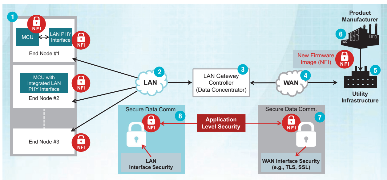
Figure 1: Example representation of network-connected MCUs in-field firmware updates
