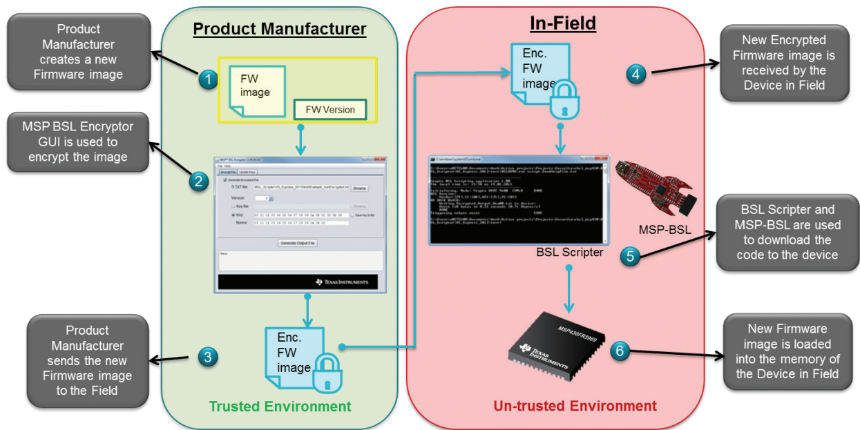
Figure 3: Crypto-Bootloader tools in in-field firmware updates flow
