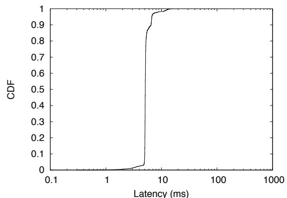
Figure 8: CDF of request latencies for 210 clients issuing 100,000 requests with Aardvark servers.
