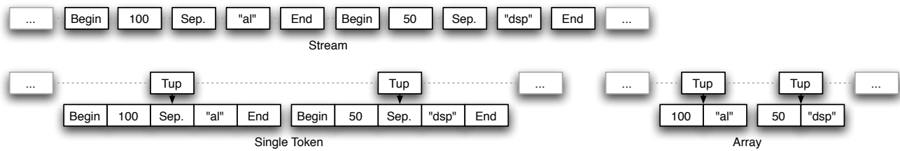
Figure 4: Tuple representations
