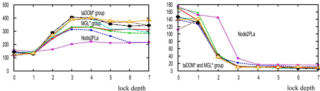
Figure 9. Synopsis of all protocols on CLUSTER1—transaction throughput (left) and deadlocks (right)
