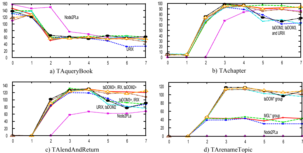
Figure 10. Transaction throughput of CLUSTER1 separated by transaction types
