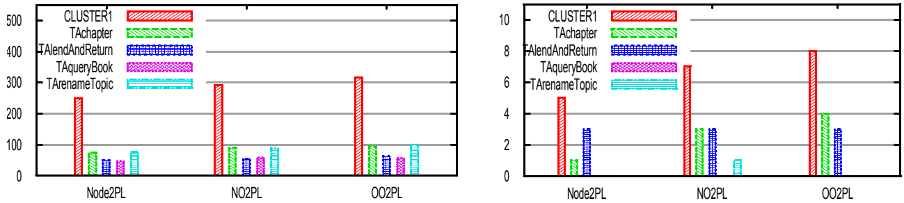
Figure 8. Running CLUSTER1 under the *-2PL group: transaction throughput (left) and deadlocks (right)
