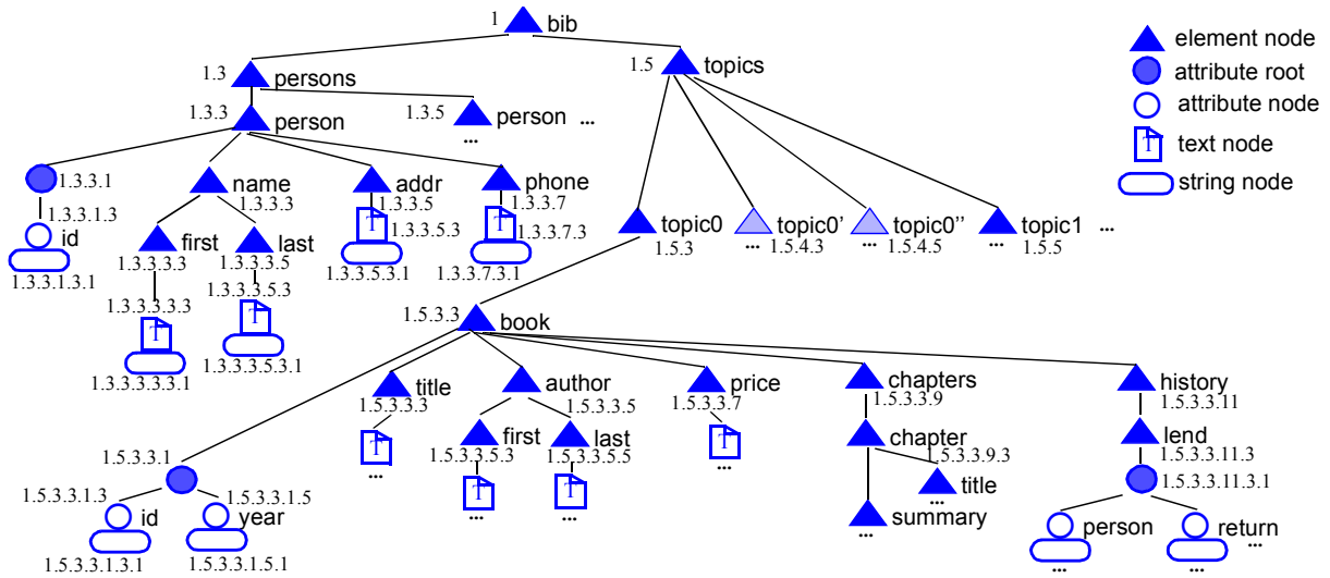
Figure 5. A sample taDOM tree of a library document labeled with SPLIDs
