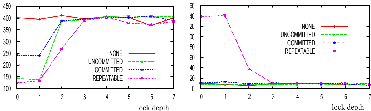
Figure 7. CLUSTER1 under taDOM3+—influence of isolation level: transaction throughput (left) and deadlocks (right)
