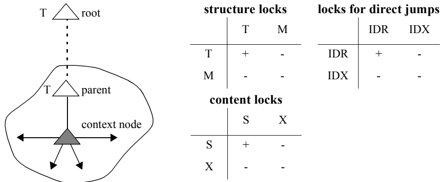
Figure 1. Node2PL sample protocol and compatibilities for the different lock types
