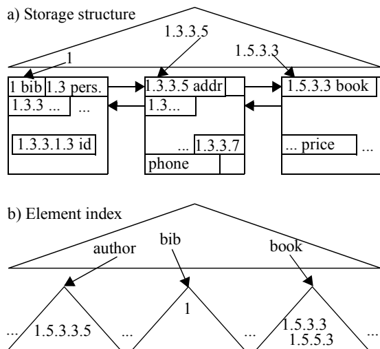
Figure 6. Document storage using B*-trees
