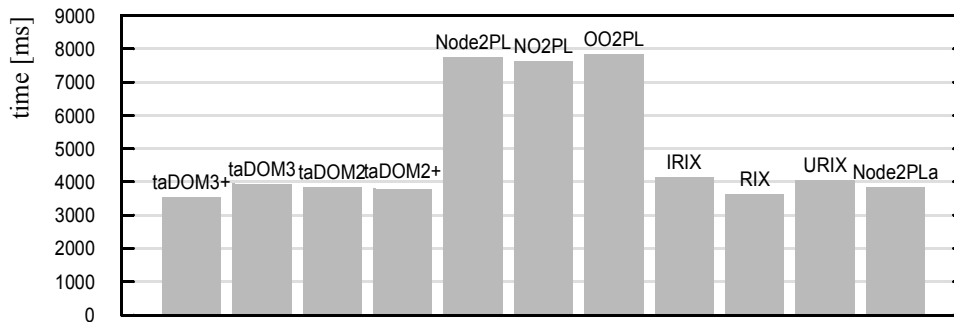
Figure 11. Transaction execution times for all protocols on CLUSTER2
