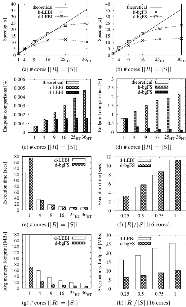
Figure 8: Comparisons for parallel processing on WEBKIT
