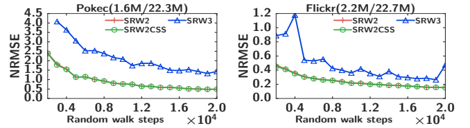
(b) 4-node clique ( \square )
