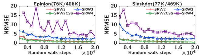
(c) 5-node clique ( \star )
