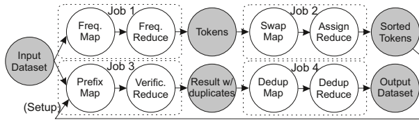
Figure 6: V-SMART Dataflow
