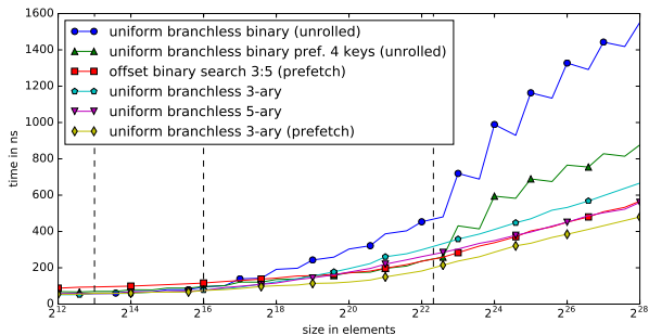
Figure 18: Fastest search algorithms on large arrays.
