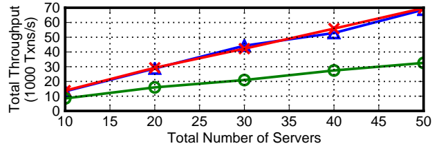
Figure 6: Scale-out of MAV, Eventual, and RC.
