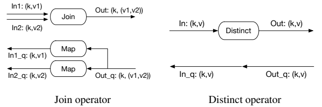
Figure 5: Optimized provenance tracking constructs
