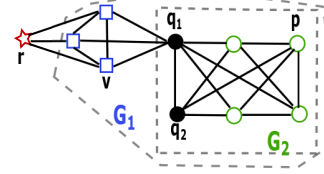
Figure 2: A graph G with Q = \{q_1, q_2\} .
