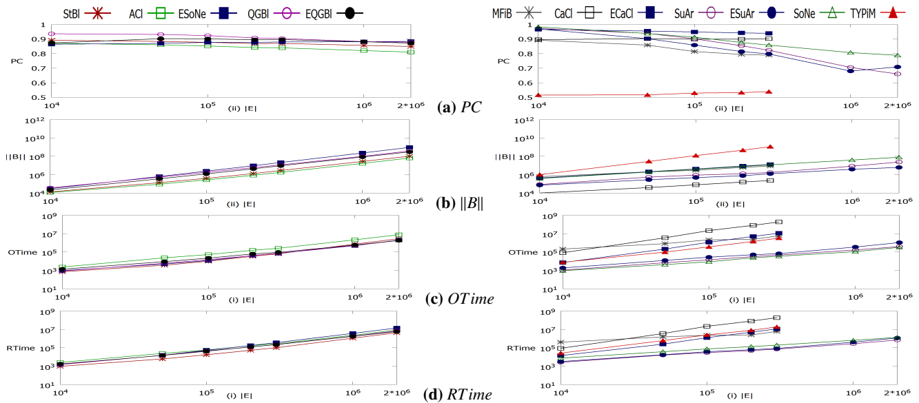
Figure 9: Scalability of the default configuration of lazy and proactive methods across the synthetic datasets with respect to (a) recall, (b) executed comparisons, (c) overhead time, and (d) resolution time. All axes are logarithmic except for the vertical ones in (a).
