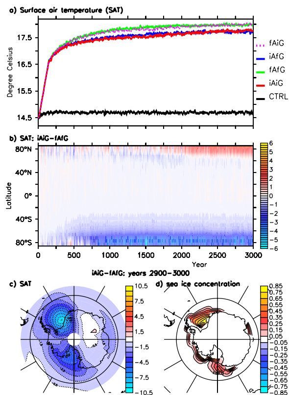
Figure 1. Time series of the annual mean surface air temperature (SAT in °C): (a) globally averaged from CTRL (black), iAiG (red), fAfG (green), iAfG (blue) and fAiG (purple dotted line) and (b) zonally averaged: difference between iAiG and fAfG. A 10-year running mean has been applied to all time series. (c) SAT difference between iAiG and fAfG averaged over years 2900 to 3000 expressed in °C and (d) same difference but for sea-ice concentration for each grid (ratio between 0 and 1), which is an index of sea-ice cover.
