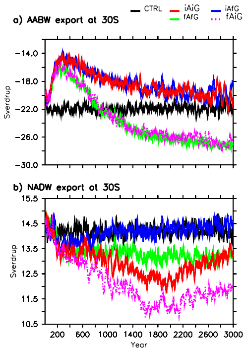
Figure 2. Time series of the annual mean value of (a) the minimum of the oceanic global meridional overturning streamfunction at 30^{\circ}\text{S} (in Sv, 1\text{ Sv} = 10^6\text{ m}^3/\text{s} ), representing the export of Antarctic and Circumpolar Deep Water (AABW and CDW) at 30^{\circ}\text{S} , and (b) the maximum of the Atlantic meridional overturning streamfunction at 30^{\circ}\text{S} , representing the export of North Atlantic Deep Water (NADW) at 30^{\circ}\text{S} . CTRL is in black, iAiG in red, fAfG in green, iAfG in blue and fAiG in purple dotted line. A 21-year running mean has been applied to all time series.
