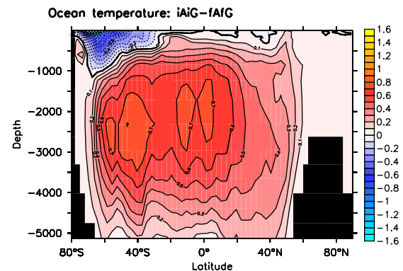
Figure 3. Latitude-depth distribution of the annually averaged temperature difference (in ^{\circ}\text{C} ), years 2900 to 3000, of iAiG minus fAfG in the global ocean. Blue (red) shading indicates values where the water is colder (warmer) in iAiG than in fAfG. The contour interval is 0.2^{\circ}\text{C} .
