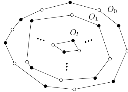
Figure 5: An onion 2-coloration and its onion layers.
