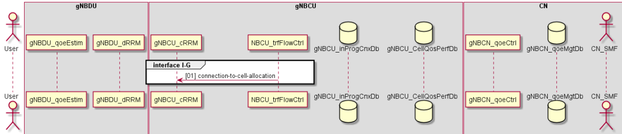
Figure 7-5: Interface IG flow chart
