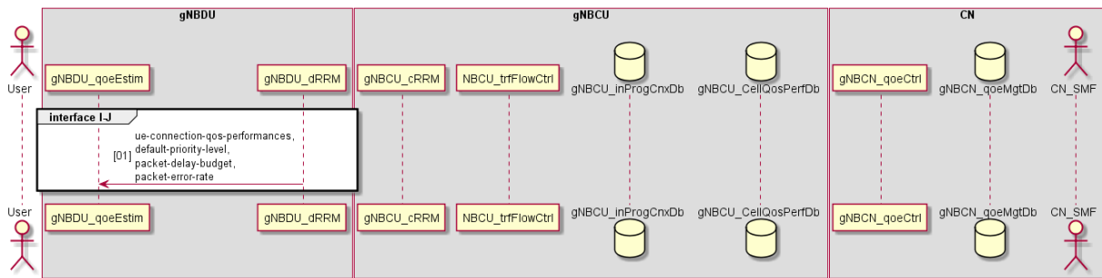
Figure 7-8: Interface IJ flow chart
