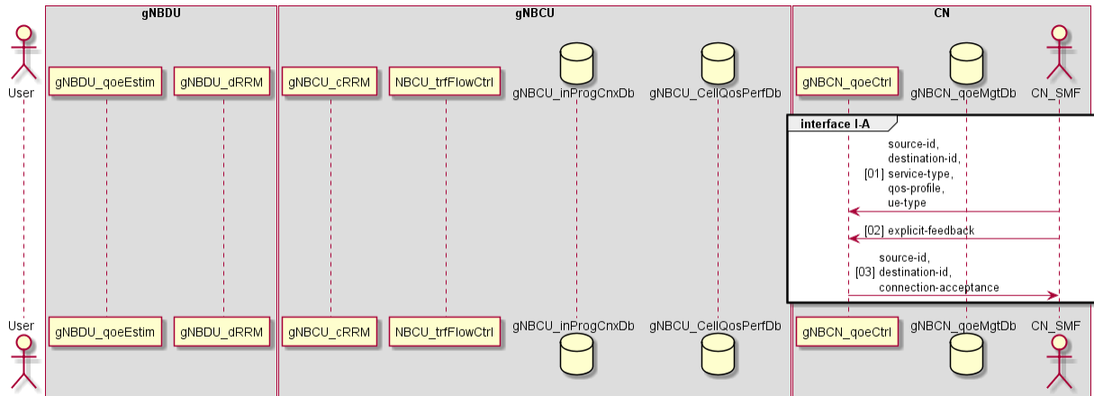
Figure 7-2: Interface IA flow chart
