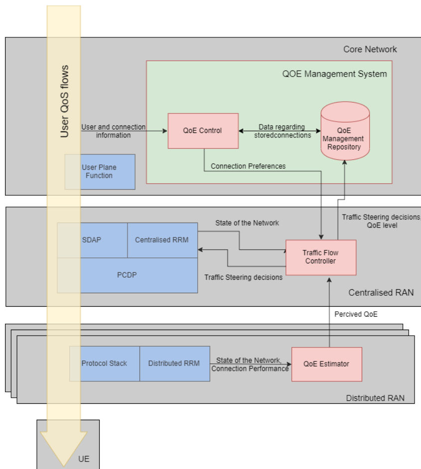
Figure 6-2: QoE management system functional architecture
