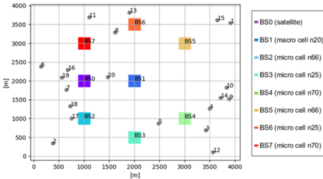
Figure 5-7 Network scenario
