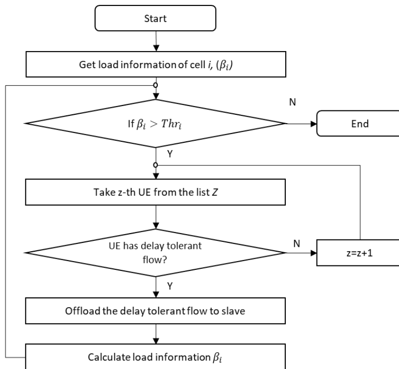
Figure 5-16: Flow diagram of proposed MLB algorithm
