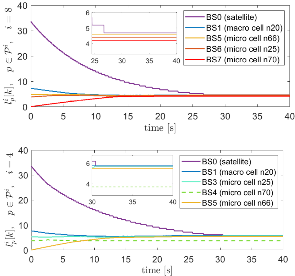
Figure 5-10: Commodity latency examples during the simulation (solid lines: unconstrained providers used by the commodity; dashed line: constrained providers; zoomed sub-plots to show the convergence within the tolerance \epsilon = 0.5 ).
