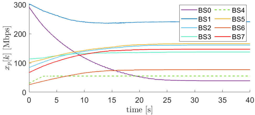
Figure 5-9 Network state in terms of total bitrate allocated on the various APs (solid lines: unconstrained providers, dashed line: constrained provider).
