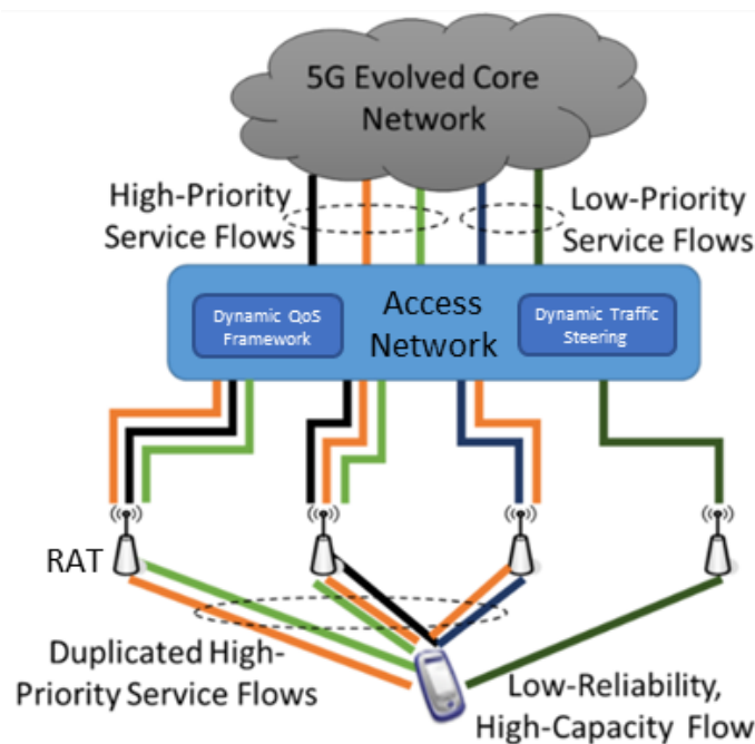
Figure 5-6: Dynamic Traffic Steering framework from [18]
