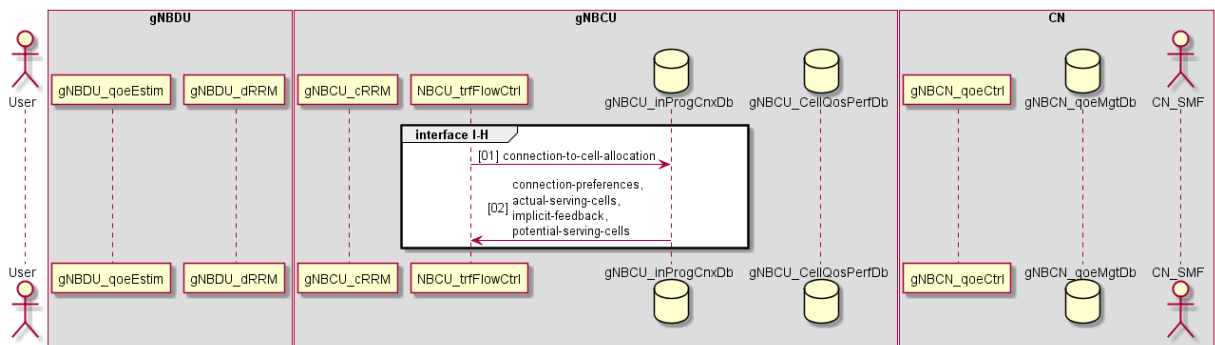
Figure 7-6: Interface IH flow chart
