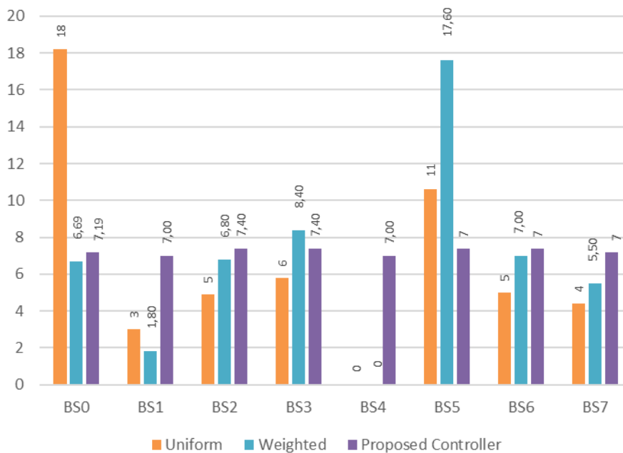
Figure 5-11 Comparison for the three considered algorithms of the latencies over APs for commodity i = 20 .
