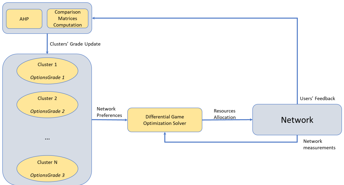
Figure 5-25 Block diagram of the AHP algorithm
