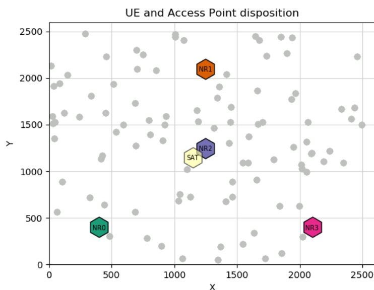
Figure 4-1 Network Simulator GUI. Scenario with 3 ground AP and a Satellite. Grey dots: UEs.
