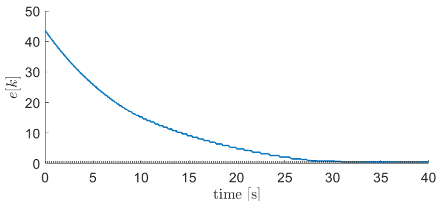
Figure 5-8 Maximum latency mismatch during the simulation (dotted line: tolerance \varepsilon ).
