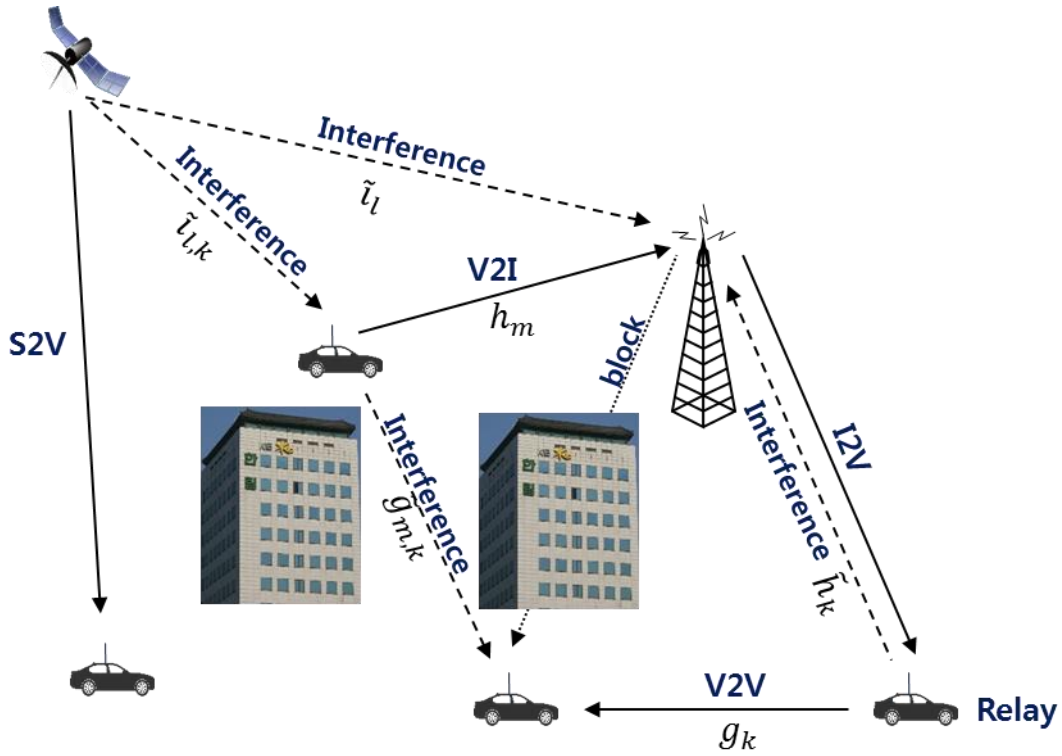
Figure 5-19: The analysis scenario for the proposed algorithm: the radio resource allocation policy with RL based interference control
