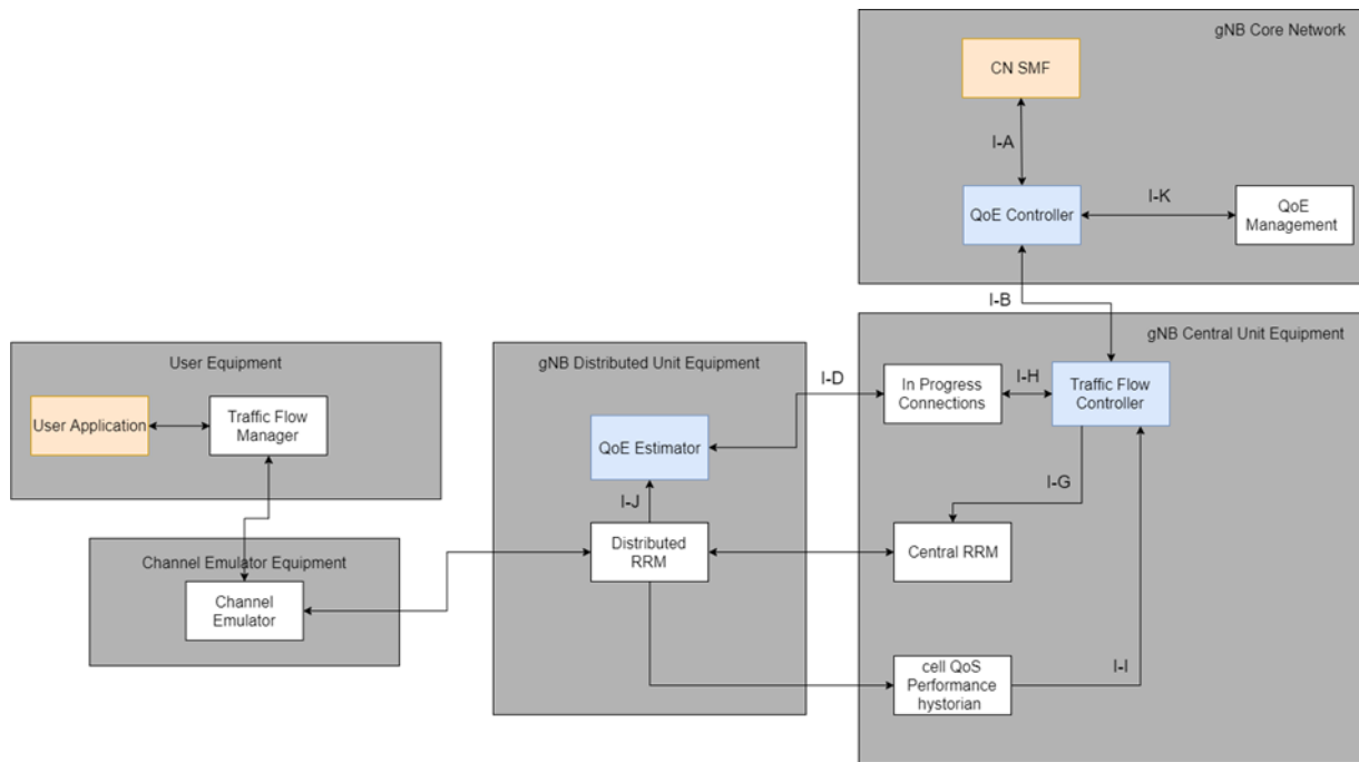
Figure 7-1: Preliminary architecture of the project EU-PoC
