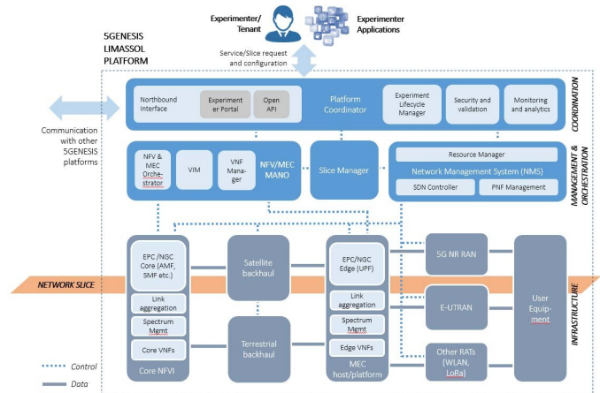
Fig. 2. Functional architecture of the 5GENESIS Limassol platform
