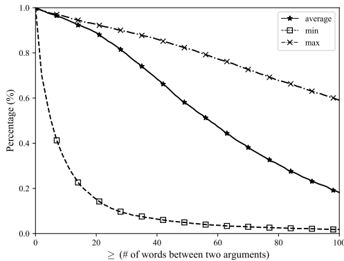
Figure 3: Number of words between two arguments within a dialogue in DialogRE.
