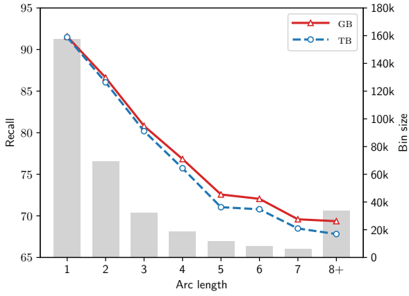
(a) Recall
