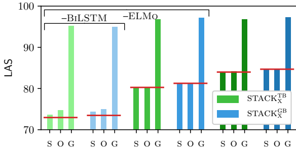
(a) Stacking with different types of level-0 information: S – self, O – other, G – gold.
