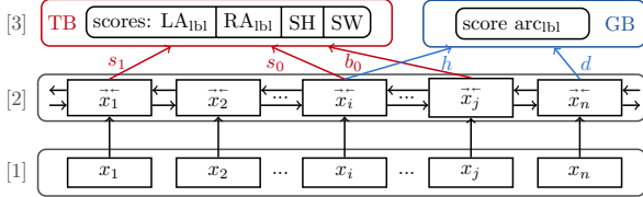
Figure 1: Architectures of BiLSTM-based dependency parsers employed in this work. Layers: [1] word representations, [2] BiLSTMs, [3] multi-layer perceptron.
