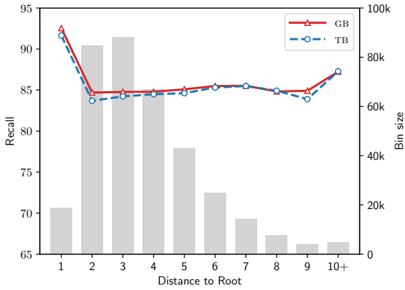
(a) Recall
