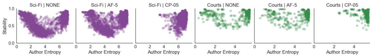
Figure 7: Topic Stability and Entropy for SCI-FI ( K = 250 ) and COURTS ( K = 50 ). AF-5 has little effect. Many of the low-entropy topics avoided by CP-05 are highly unstable.
