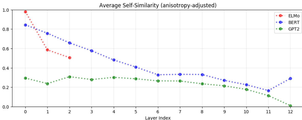
Figure 2: The average cosine similarity between representations of the same word in different contexts is called the word’s self-similarity (see Definition 1). Above, we plot the average self-similarity of uniformly randomly sampled words after adjusting for anisotropy (see section 3.4). In all three models, the higher the layer, the lower the self-similarity, suggesting that contextualized word representations are more context-specific in higher layers.
