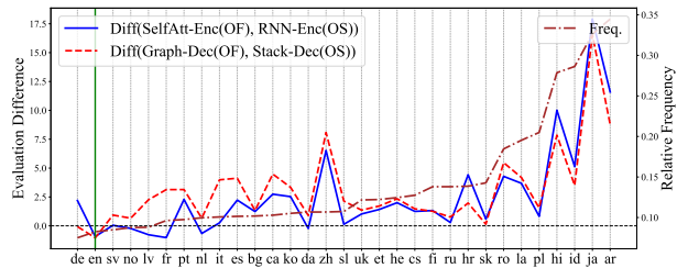
Figure 4: Evaluation differences of models on d=1 dependencies. Annotations are the same as in Figure 3, languages are sorted by percentages (represented by the brown curve and right y -axis) of d=1 dependencies.
