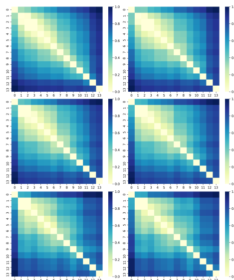
Figure 3: Normalised sum squared errors when aligning the word vectors across different years (2000–2013), using the complete vocabulary (left) and the its intersection with the OED dictionary (right), with different minimum frequency thresholds: 1K (top), 10K (middle) and 100K (bottom).
